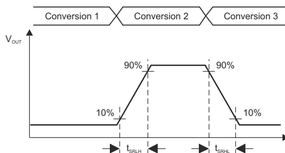
图 8-22. Slew Rate Testing
