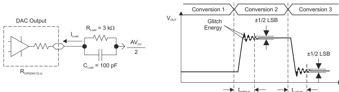
图 8-21. Settling Time and Glitch Energy Testing
