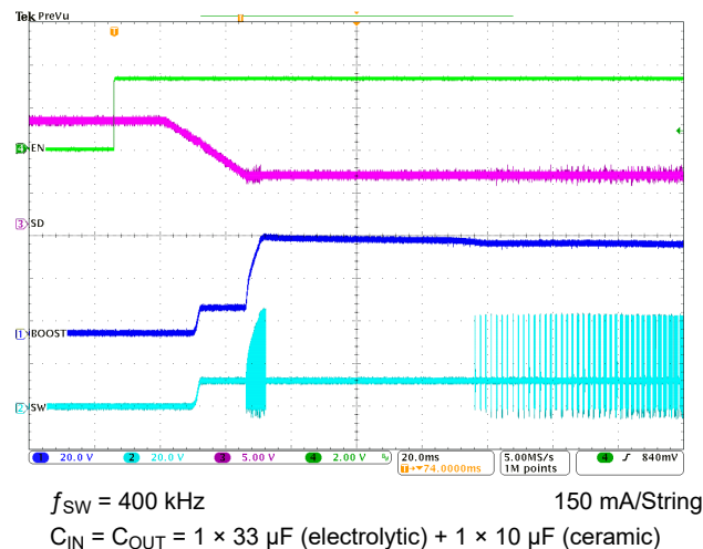
图 8-4. Typical Start-Up
