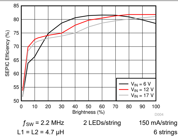
图 6-5. SEPIC Efficiency
