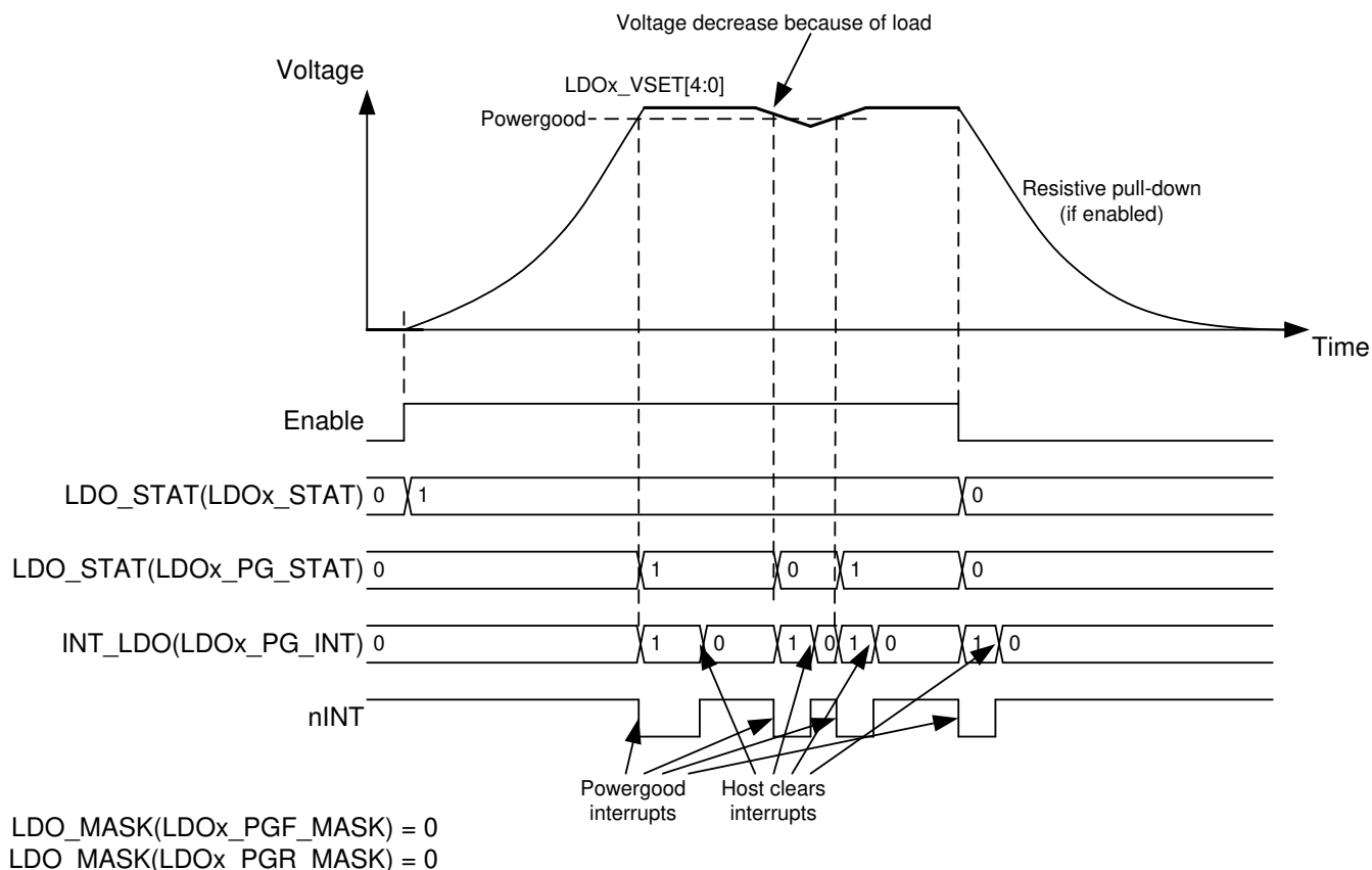
图 7-5. LDO Regulator Enable and Disable
