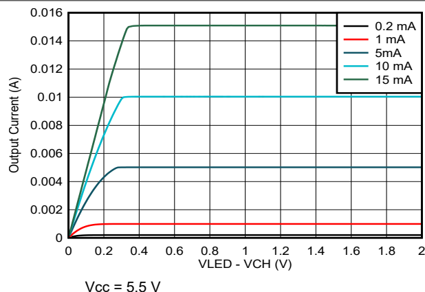
图 7-3. Channel Current vs (VLED-Vchannel) Voltage
