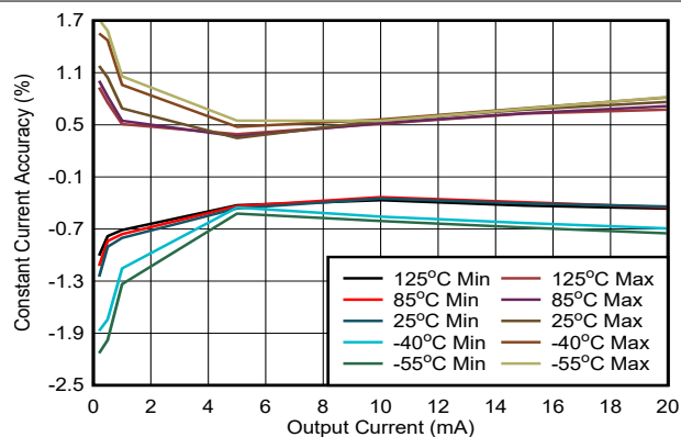
图 7-5. Channel to Channel Accuracy vs Output Current
