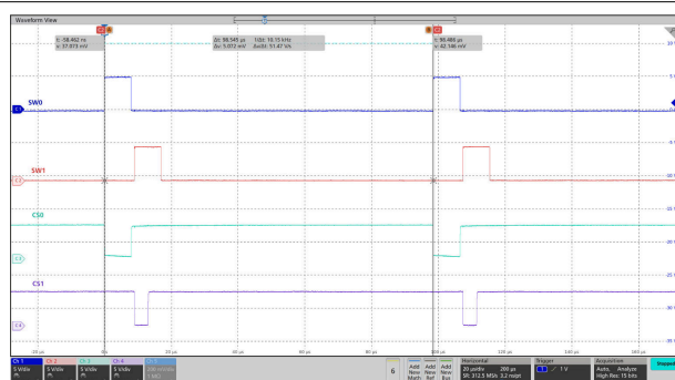
图 9-3. Scan Lines and Current Sinks Waveforms of SW0, SW1, CS0, CS1
