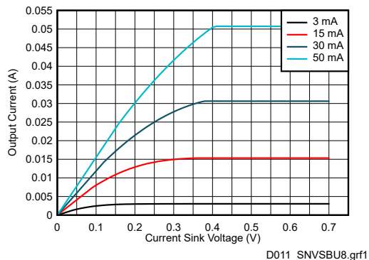
图 7-7. Current Sinks Voltage vs Current
