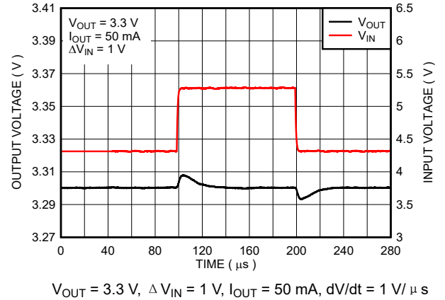
图 8-6. Line Transient Response for New Chip
