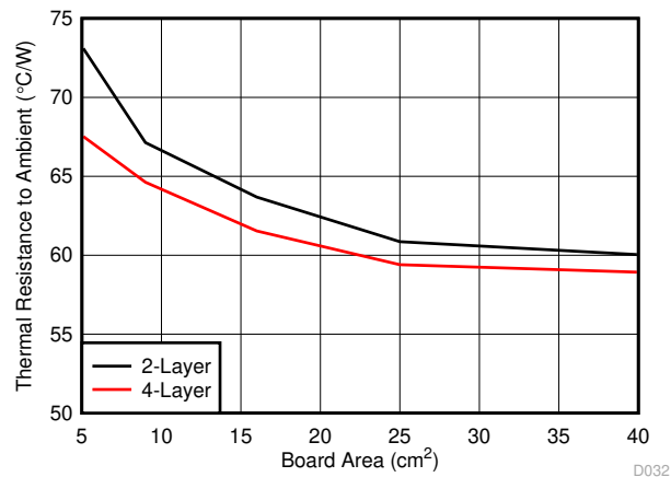
图 9-48. Package Thermal Resistance vs Board Copper Area
