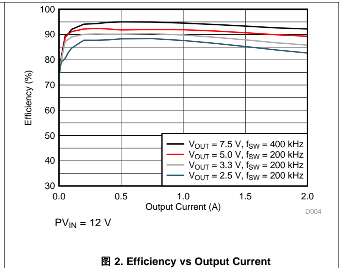
图 2. Efficiency vs Output Current
