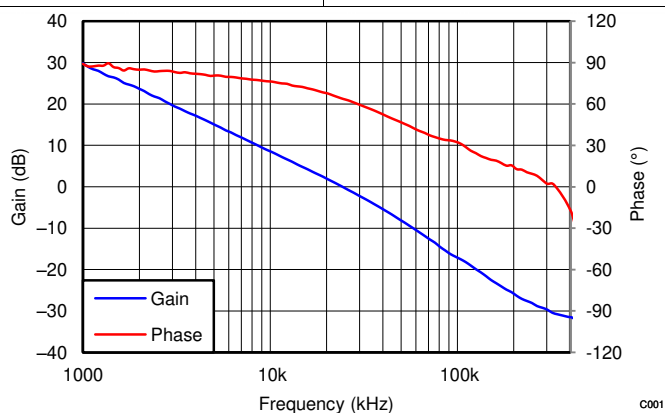
Figure 15. V OUT = 1.8 V, I OUT = 7 A, C OUT = 200 μF Ceramic, f sw = 500 kHz
