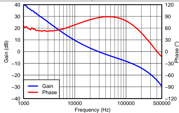
Figure 5. VOUT = 1.8 V, IOUT = 4 A, COUT1 = 47 µF ceramic, COUT2 = 100 µF POSCAP, fSW = 1 MHz
