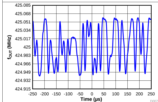
图 19. 4-Level GFSK Modulation
