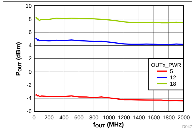
图 17. Output Power vs Frequency
