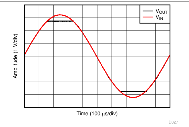
G = 1 , V_{IN} = 6.5\text{V}_{PP}
