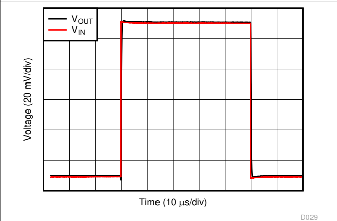
G = 1 , V_{IN} = 100\text{mV}_{PP} , C_L = 10\text{pF}
