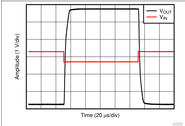
G = -10 , V_{IN} = 600\text{mV}_{PP}
