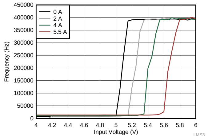
Figure 19. Frequency Dropout Characteristics ( V_{OUT} = 5\text{ V} )
