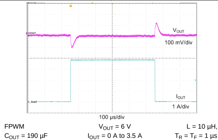
Figure 51. Load Transient
