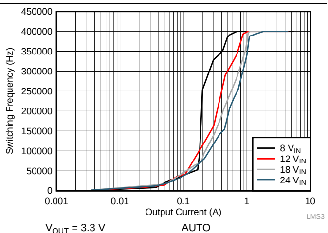
Figure 43. Switching Frequency vs Load Current
