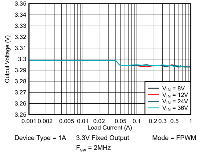
Figure 8-3. Load Regulation
