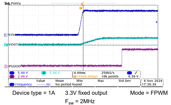
Figure 8-5. Start-up
