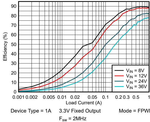
Figure 8-2. Efficiency
