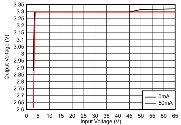
LMR36500P3 V_{OUT} = 3.3V (固定值) 1MHz (FPWM)
