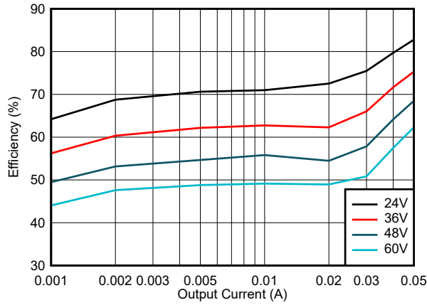
LMR36500P V_{OUT} = 12V (调整) 1MHz (自动)
