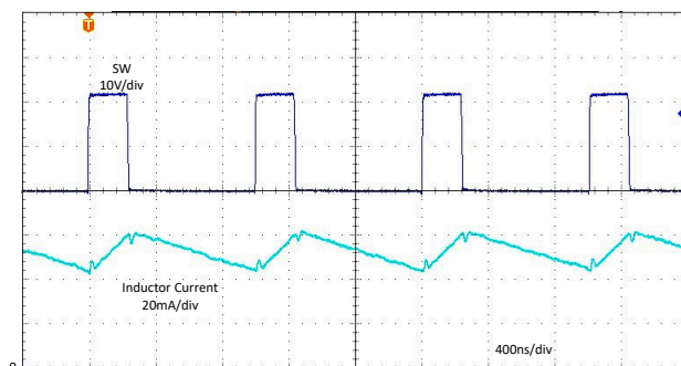
LMR36500P5 V_{OUT} = 5V 1MHz (自动) V_{IN} = 24V I_{out} = 50mA
