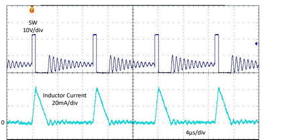
LMR36500P5 V_{OUT} = 5V 1MHz (自动) V_{IN} = 24V 输出电流 = 5mA
