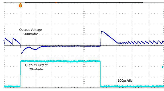
LMR36500P V_{OUT} = 1.8V (调整) 1MHz (自动) V_{IN} = 12V I_{out} = 5mA 至 50mA
