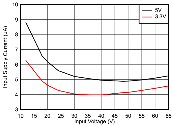
LMR36500P (固定) I_{OUT} = 0mA 1MHz (自动)
