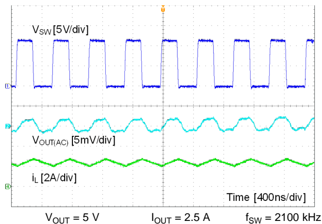
Figure 23. CCM Mode
