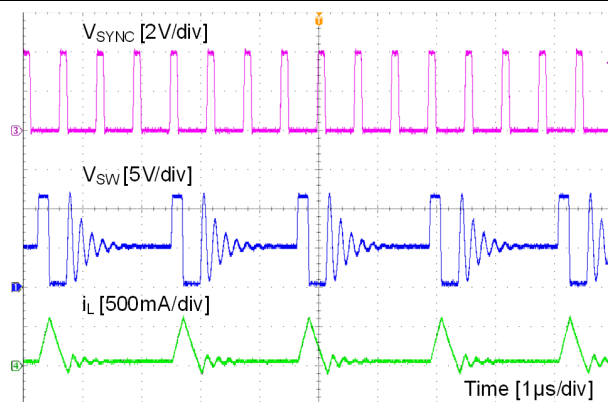
Figure 18. Synchronizing in PFM Mode
