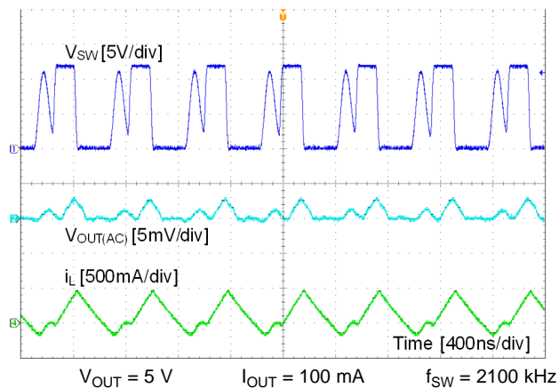
Figure 24. DCM Mode
