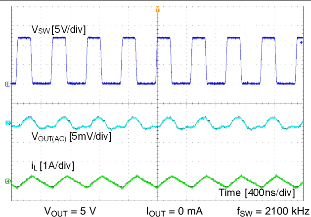
Figure 26. FPWM Mode
