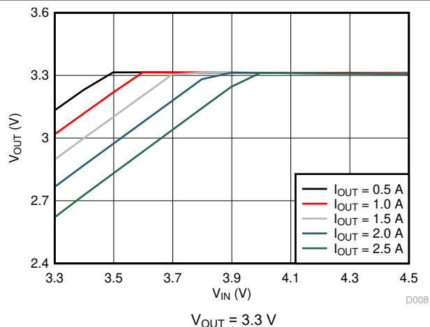
图 6-8. Dropout Curve
