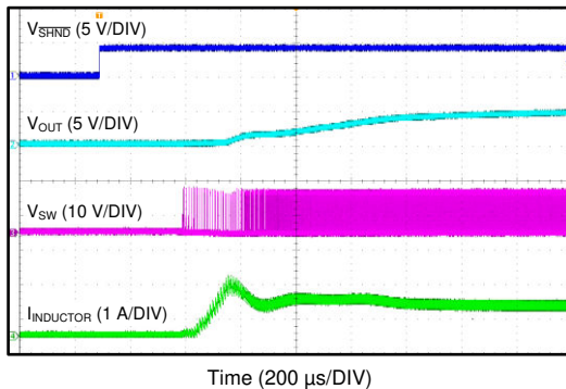
图 7-6. Start-Up Waveform ( V_{IN} = 12\text{ V} , V_{OUT} = 5\text{ V} , I_{Load} = 800\text{ mA} )
