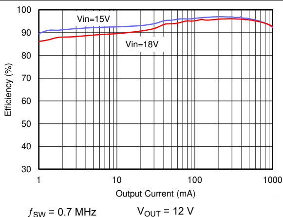
图 5-1. Efficiency vs Load Current
