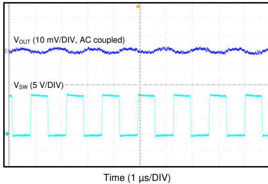
图 7-2. Switching Node and Output Voltage Waveform ( V_{IN} = 12\text{ V} , V_{OUT} = 5\text{ V} , I_{Load} = 1\text{ A} )
