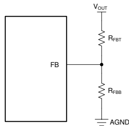
图 8-6. Setting Output Voltage for Adjustable Output Variant
