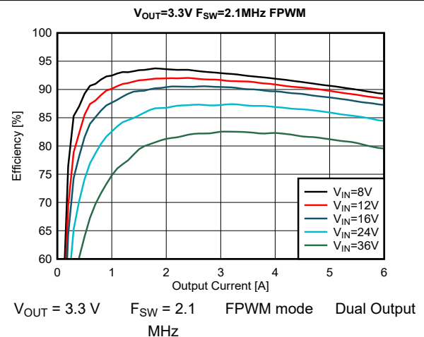
图 9-26. Efficiency
