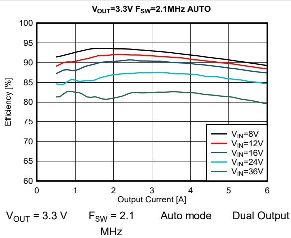
图 9-25. Efficiency
