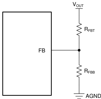
图 8-3. Setting Output Voltage of Adjustable Versions
