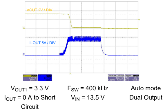
图 9-42. Short-Circuit Protection
