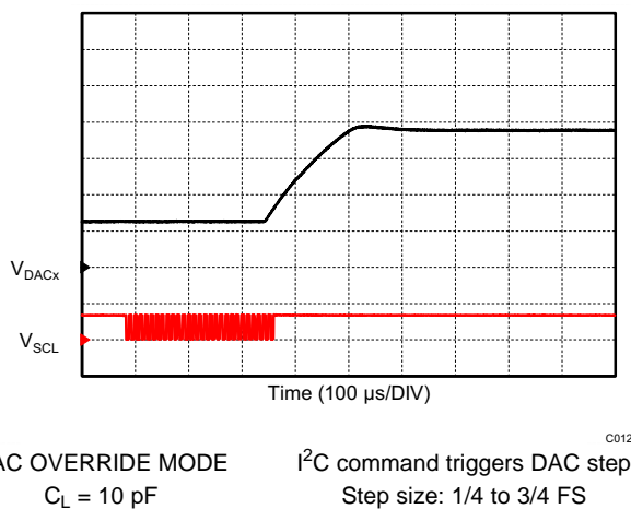
Figure 14. DAC Step Response
