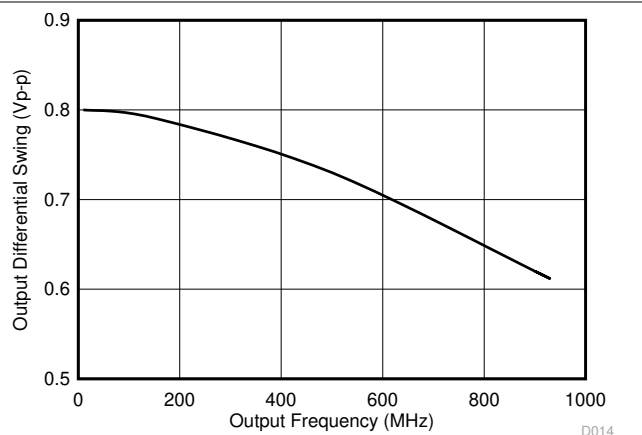
图 6-14. LVDS Differential Output Swing vs Frequency
