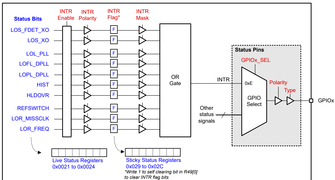
图 9-22. Status and Interrupt
