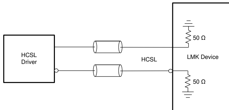
图 9-14. HCSL (Load Terminated) to Reference (INx)
