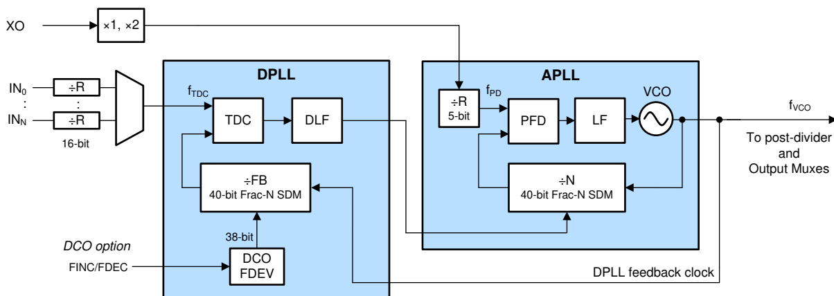
图 9-23. PLL Architecture
