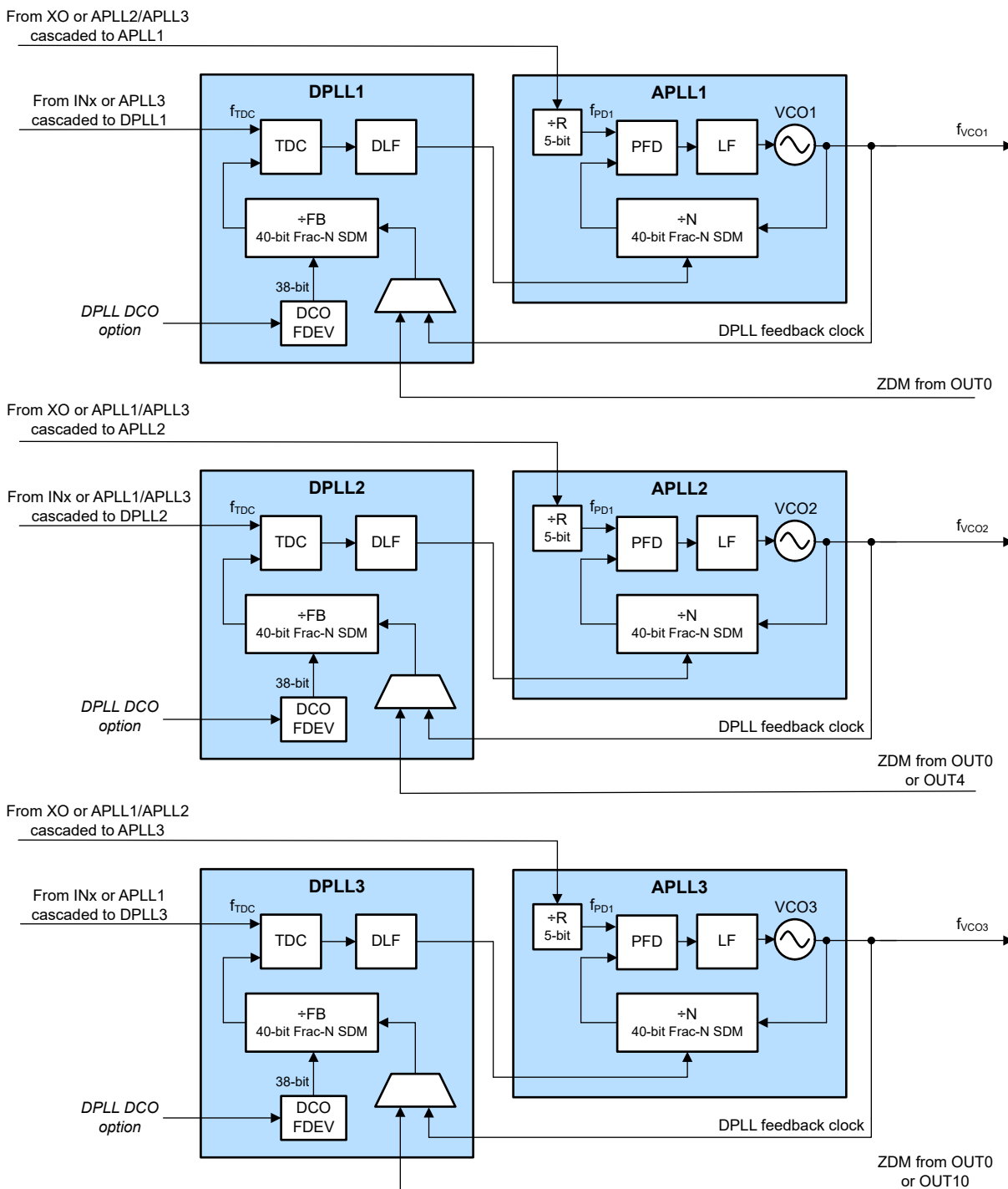
图 9-2. PLL Architecture
