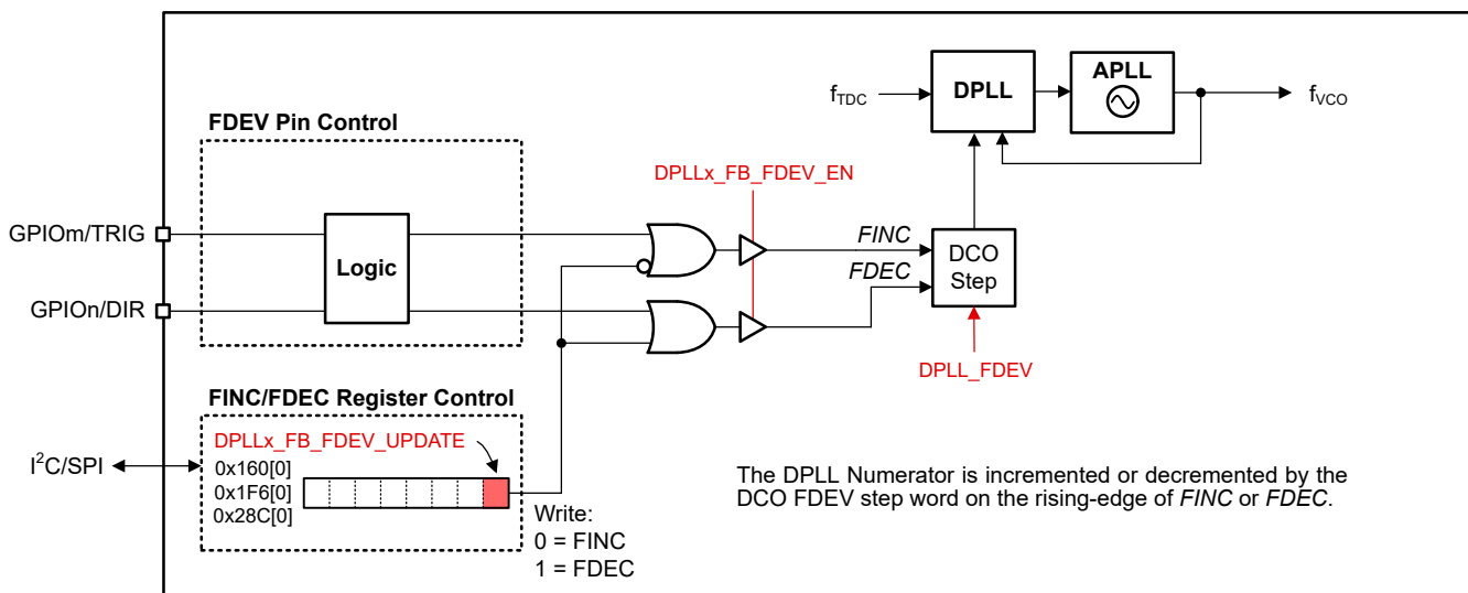
图 8-39. DCO Mode Control Options
