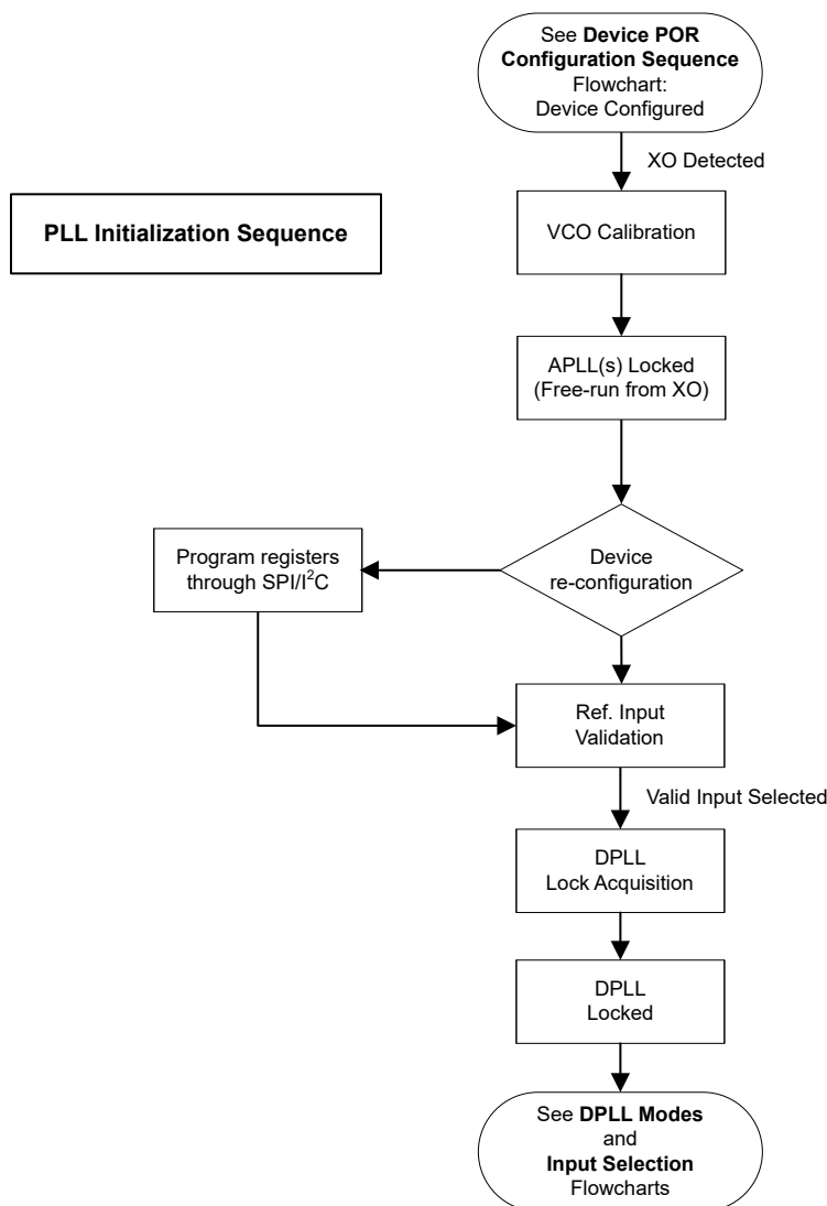
图 8-38. PLL Initialization Sequence
