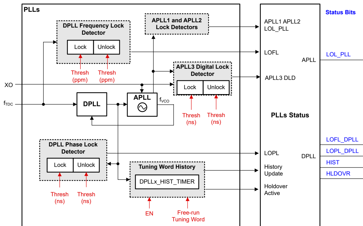
图 8-18. PLL Lock Detectors and History Monitor
