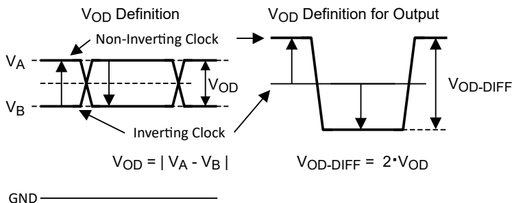
图 7-2. Two Different Definitions for Differential Output Signals
