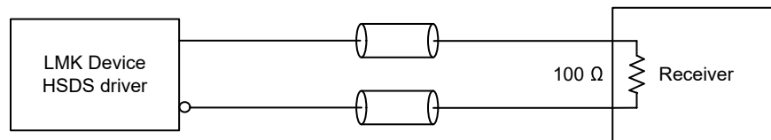
图 8-25. DC-Coupled HSDS Output Termination
