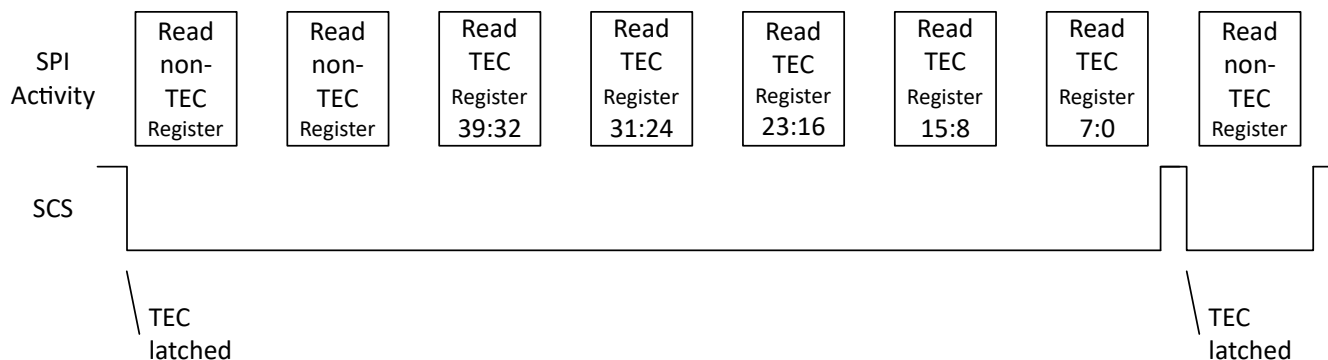
图 8-34. TEC Multibyte Read
