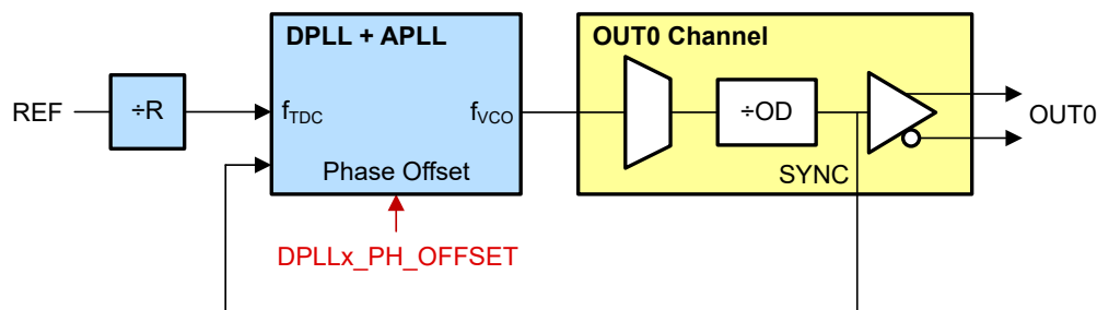
图 8-30. DPLL ZDM Synchronization Between Reference Input and OUT0
