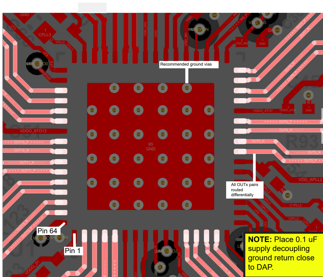
图 9-18. PCB Layout Example for LMK5B33414, Top Layer
