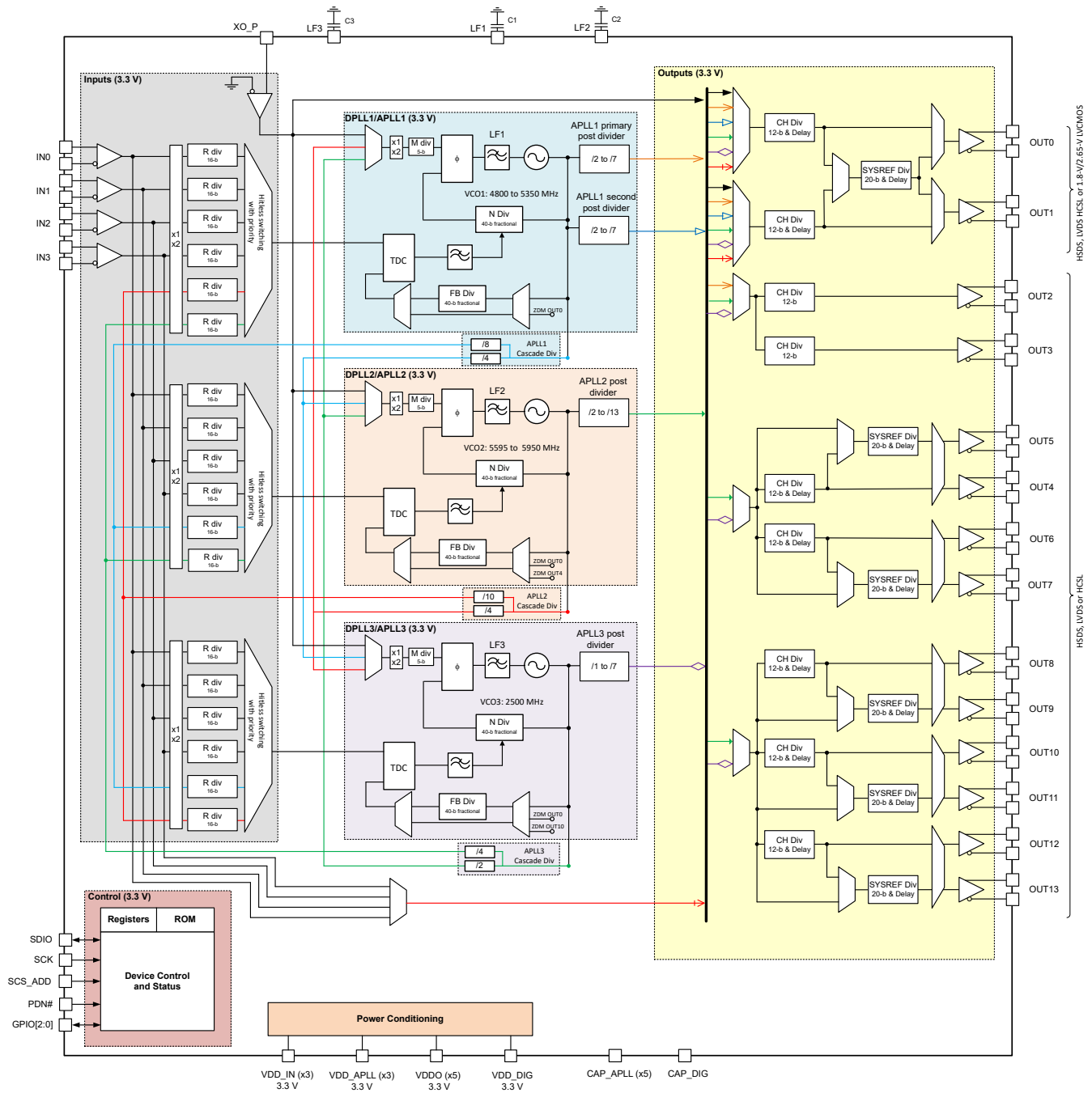
图 8-1. Top-Level Block Diagram
