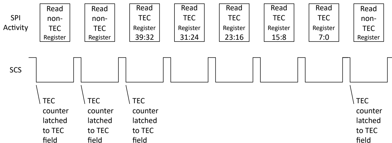
图 8-33. TEC Single Byte Read
