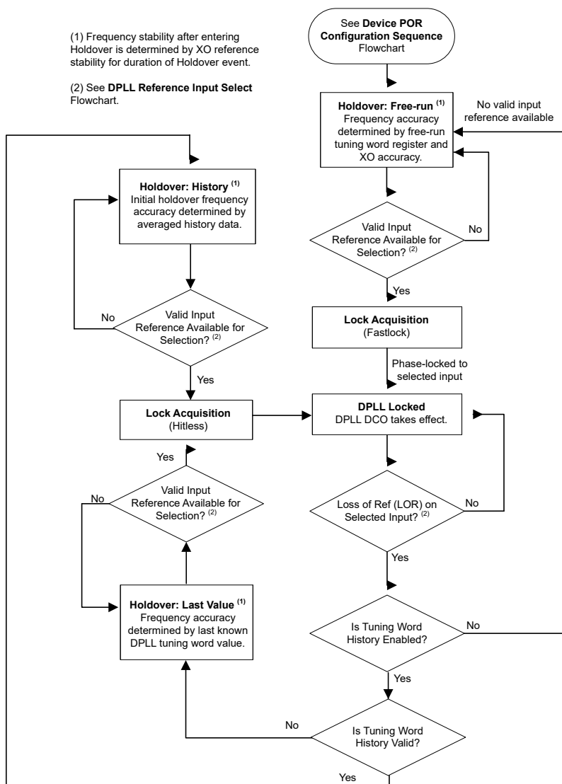
图 8-37. DPLL Operating States
