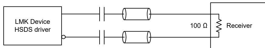
图 8-26. AC-Coupled HSDS Output Termination Method 1
