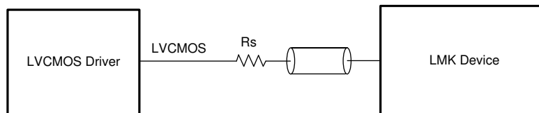
图 8-10. Single-Ended LVCNOS (1.8 V, 2.5 V, 3.3 V) to Reference (INx_P) or XO Input (XO)
