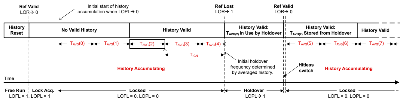
图 8-19. Tuning Word History Windows
