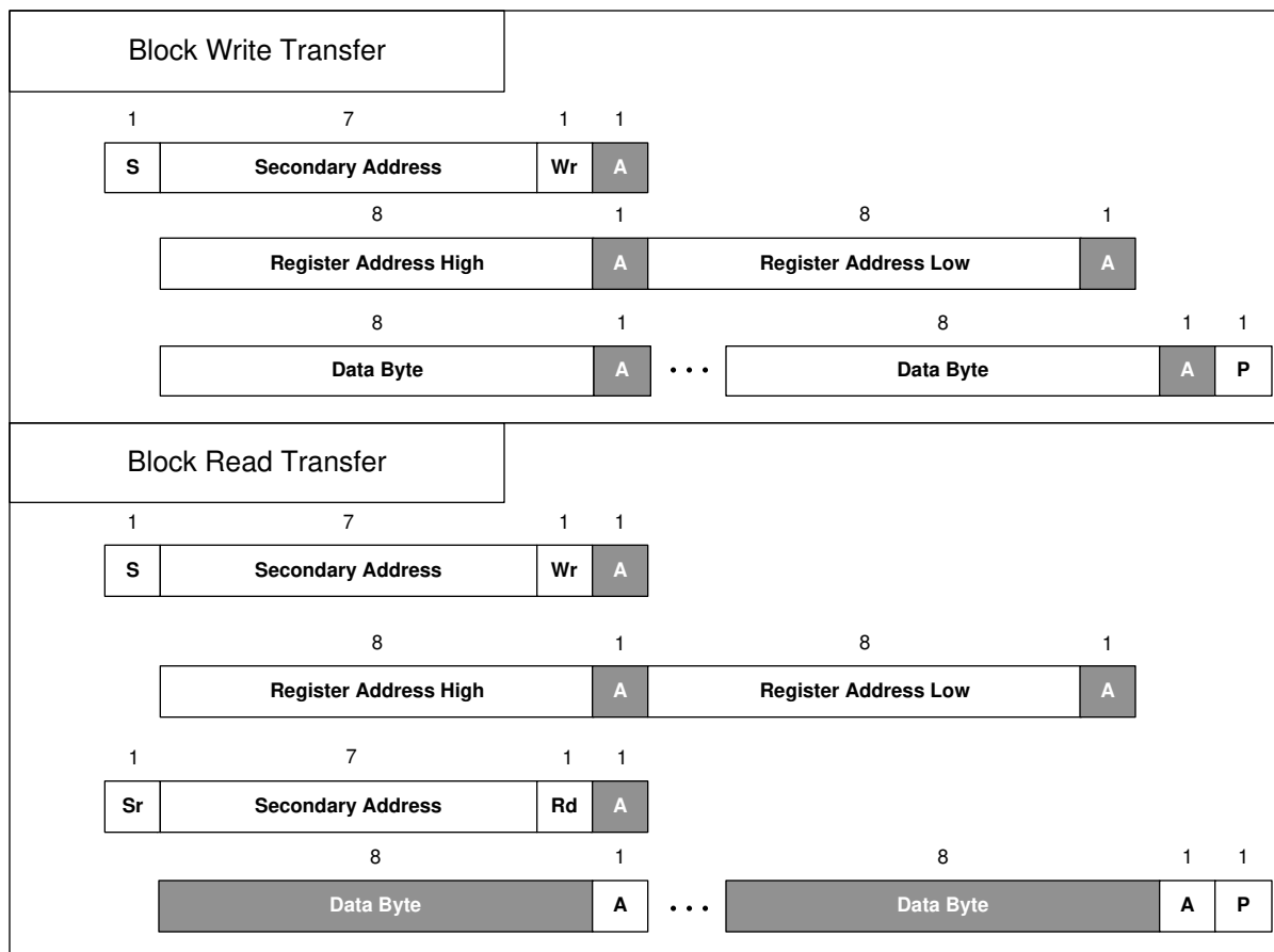
图 8-42. I 2 C Block Register Transfers
