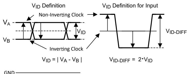
图 7-1. Two Different Definitions for Differential Input Signals
