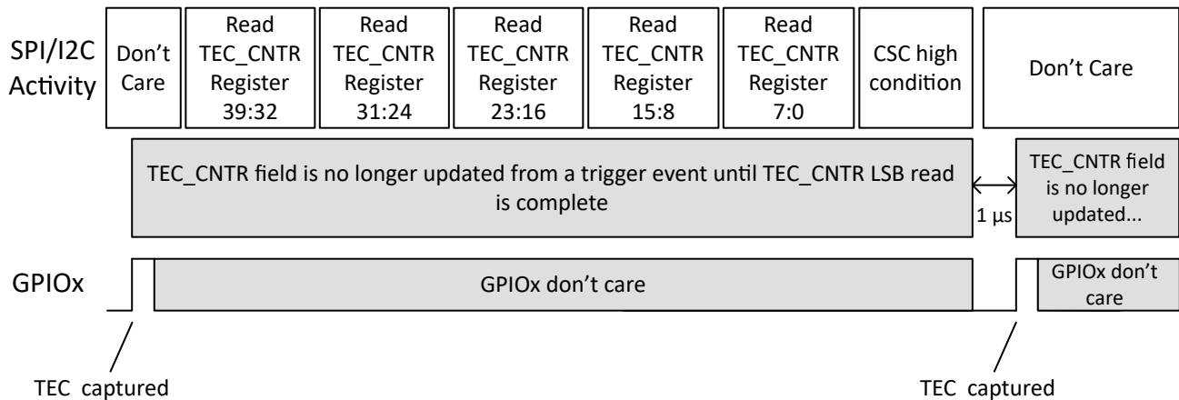
图 8-35. TEC Captured Using GPIO
