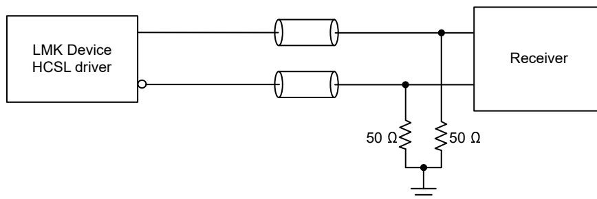
图 8-28. DC-Coupled HCSL Output Termination
