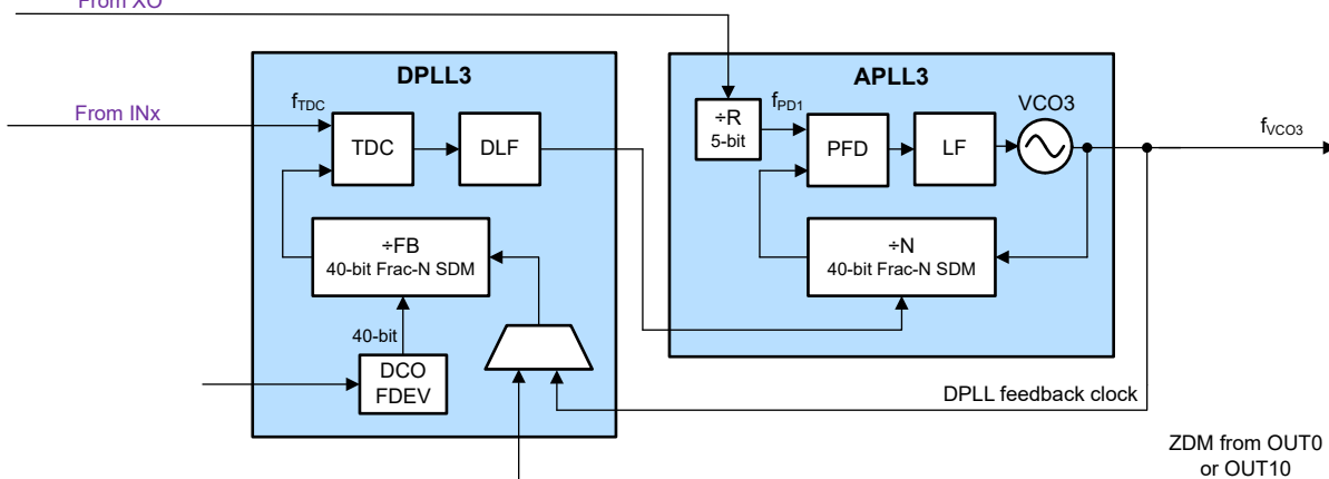
图 8-6. APLL Cascaded With DPLLs Disabled Example
