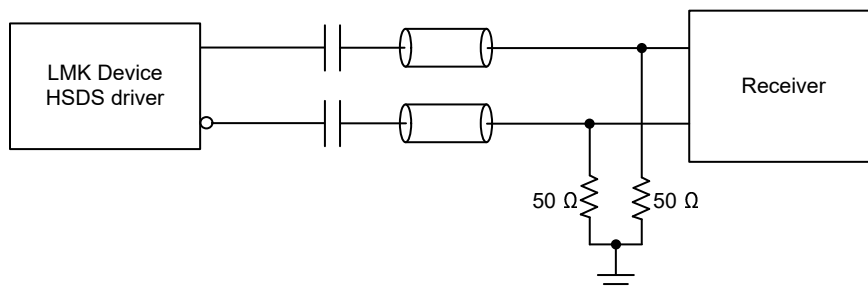
图 8-27. AC-Coupled HSDS Output Termination Method 2
