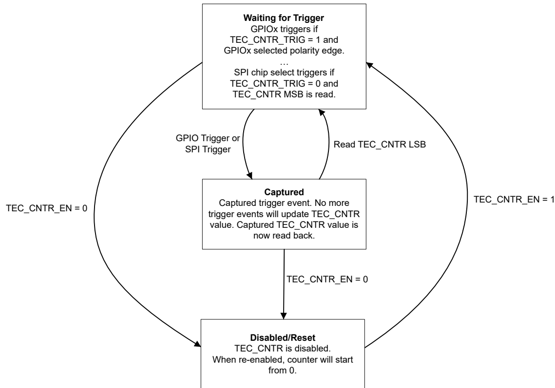
图 8-32. State Diagram of TEC
