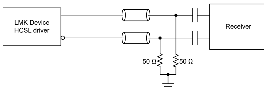
图 8-29. AC-Coupled HCSL Output Termination
