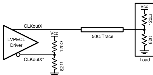
Figure 34. Single-Ended LVPECL Operation, DC Coupling, Thevenin Equivalent
