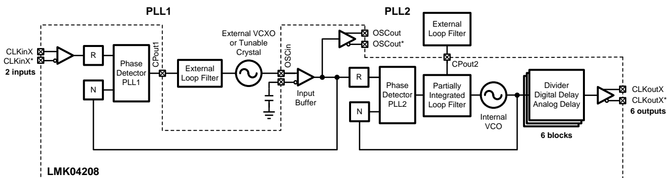
Figure 38. Simplified Functional Block Diagram for Dual Loop Mode
