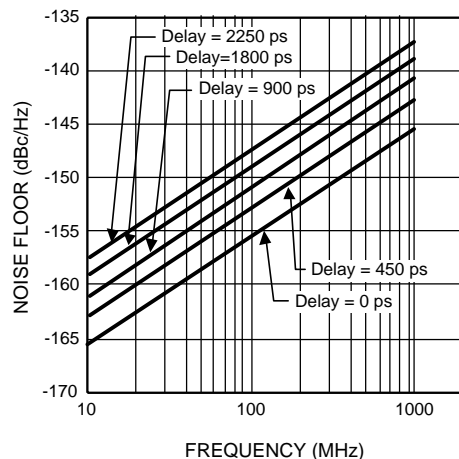
To estimate this noise, only the output frequency is required. Divide value and input frequency are not integral. The noise of the delay block is independent of output type and only applies if the delay is enabled. The noise floor due to the distribution section accounting for the delay noise can be calculated as: \text{Total Output Noise} = 10 \times \log(10^{\text{Output Buffer Noise}/10} + 10^{\text{Delay Noise Floor}/10}) . Figure 4-5. Delay Noise Floor
