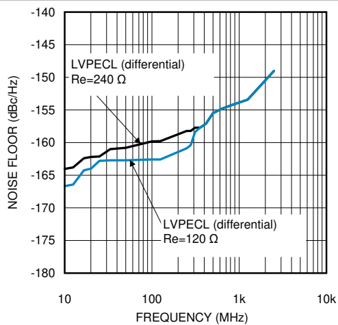
图 7-6. LVPECL Noise Floor vs. Frequency
