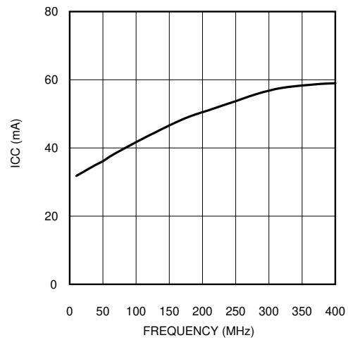
图 7-5. Typical Dynamic I_{CC} , C_L = 5\text{ pF}
