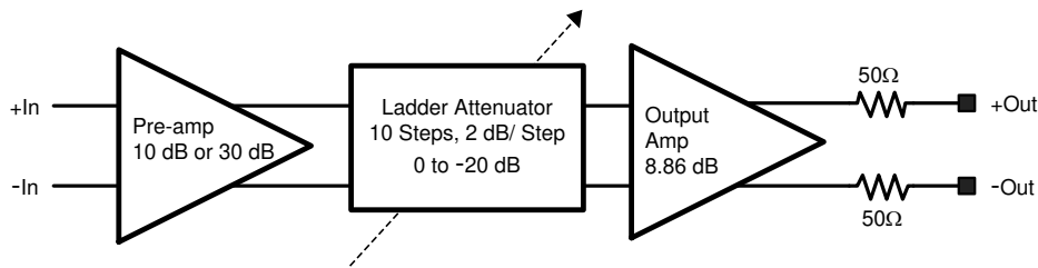
图 7-2. LMH6518 Signal Path Block Diagram
