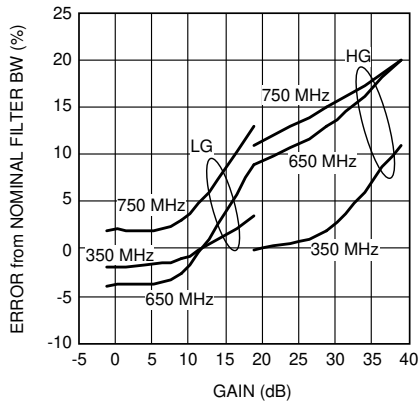
图 5-49. Filter BW vs Gain
