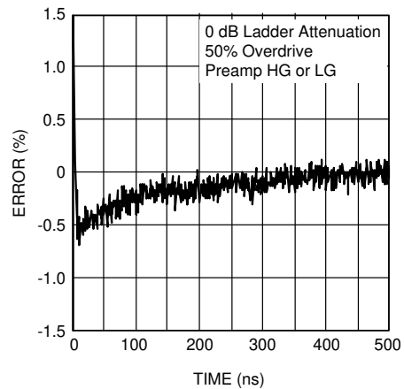
图 7-10. Overdrive Recovery
