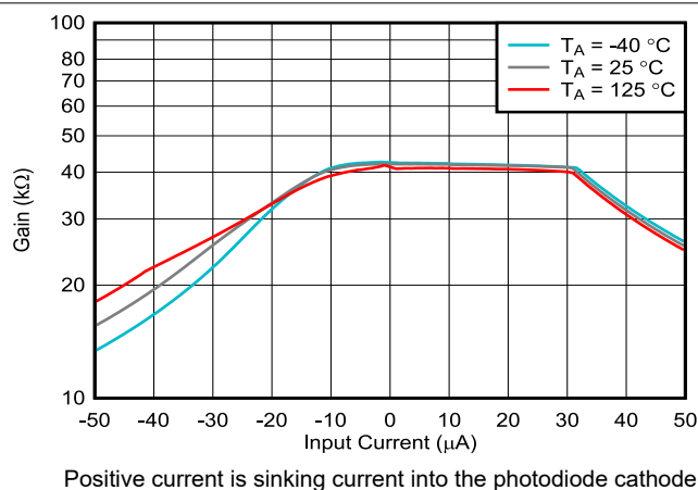
图 5-16. Transimpedance Gain vs Input Current
