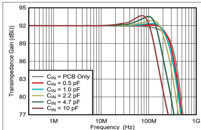
图 7-3. Small-Signal Response vs Input Capacitance
