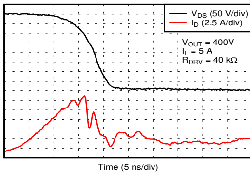
图 8-5. Turn-On Waveform in Application Example
