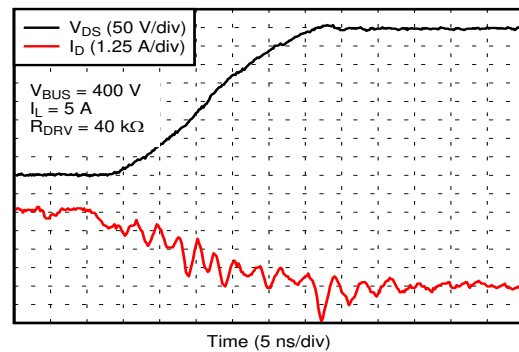
图 8-6. Turn-Off Waveform in Application Example
