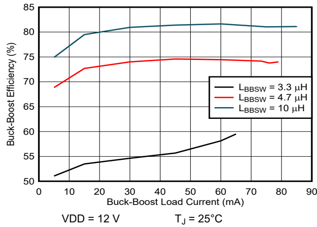
图 8-3. Buck-Boost Efficiency vs Load When I_{BBSW,PK} = I_{BBSW,PK(low)}
