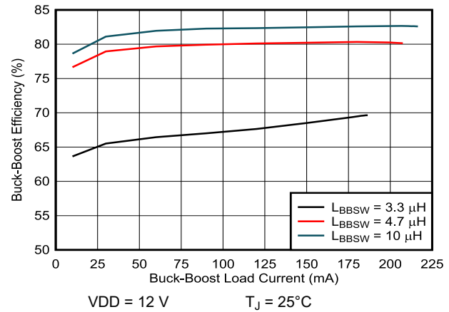
图 8-4. Buck-Boost Efficiency vs Load When I_{BBSW,PK} = I_{BBSW,PK(high)}
