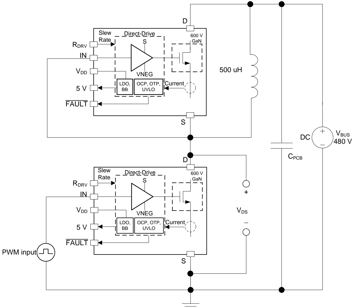
图 1. Circuit Used to Determine Switching Parameters
