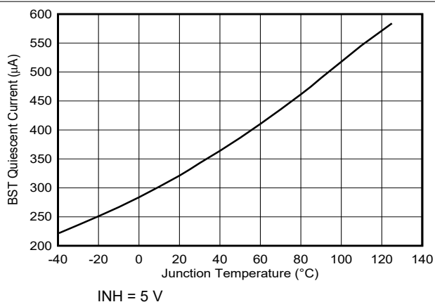
图 6-22. BST Quiescent Current vs Junction Temperature
