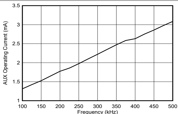
图 6-20. AUX Operating Current vs Frequency
