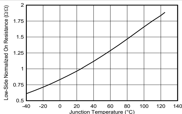
图 6-1. Low-Side Normalized On-Resistance vs Junction Temperature
