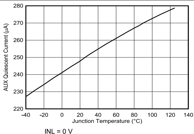
图 6-18. AUX Quiescent Current vs Junction Temperature
