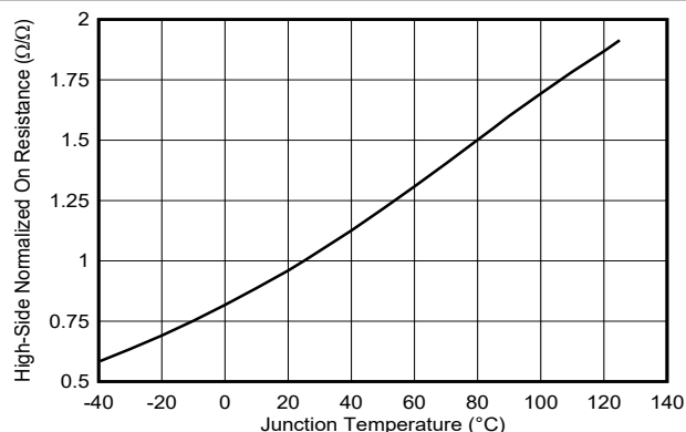
图 6-2. High-Side Normalized On-Resistance vs Junction Temperature
