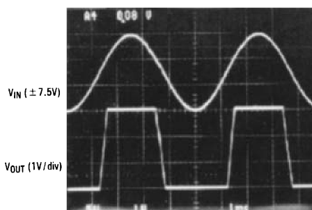
Figure 57. A \pm 7.5\text{V} Input Signal Greatly Exceeds the 3V Supply in Figure 56 Causing No Phase Inversion Due to R_I
