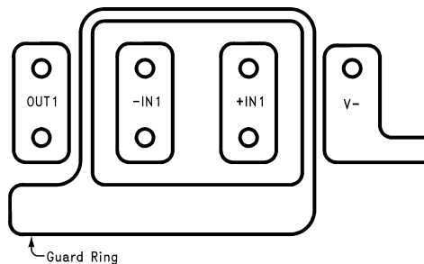
图 6-8. Example of Guard Ring in Printed Circuit Board Layout
