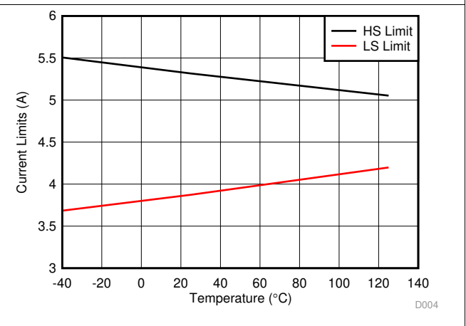
图 4. LM76003 High-Side and Low-Side Current Limits
