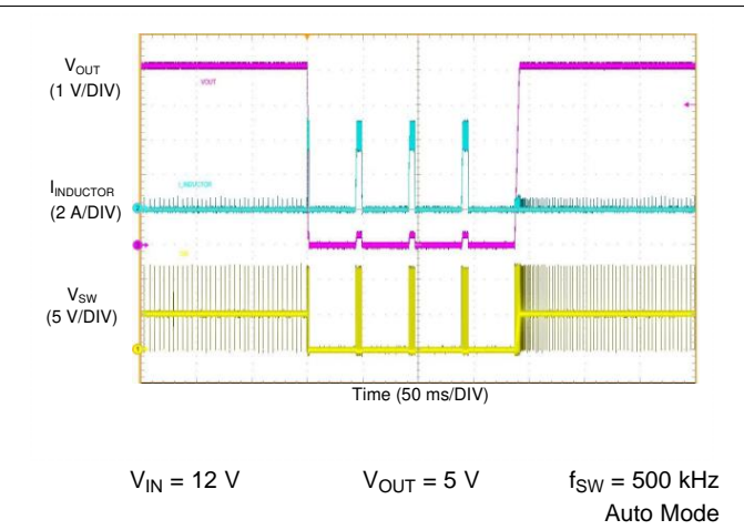
图 72. LM76003 Short-Circuit Behavior With Hiccup
