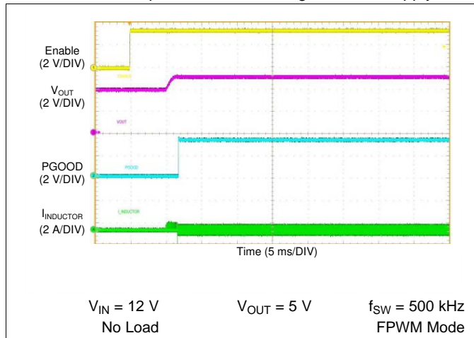
图 71. LM76002 Start-up With Pre-Biased Output
