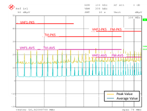
图 9-64. LM73606-Q1 Conducted EMI Result versus CISPR25 Limits - High Frequency
