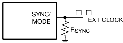
图 8-13. Frequency Synchronization
