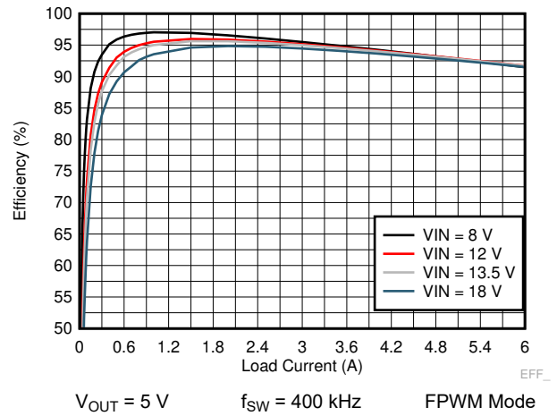
图 9-12. LM73606-Q1 Efficiency
