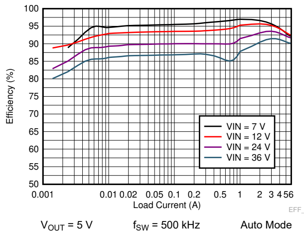
图 9-13. LM73606-Q1 Efficiency
