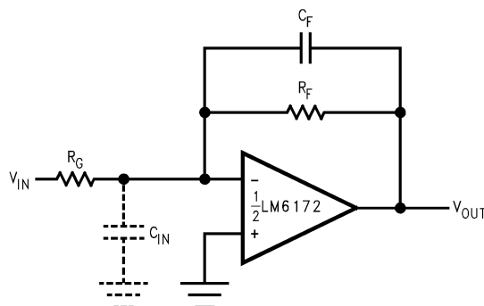
Figure 46. Compensating for Input Capacitance
