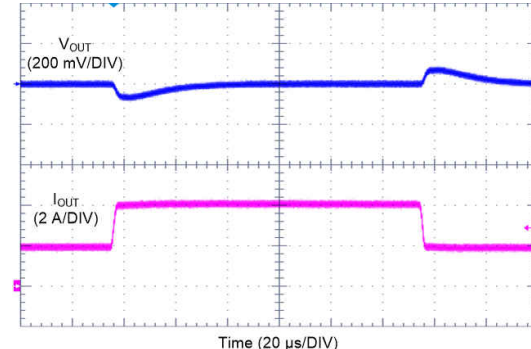
Time (20 µs/DIV) V_{OUT} = 3.3\text{ V} F_{SW} = 2100\text{ kHz} AUTO Mode I_{OUT} = 2\text{ A to } 4\text{ A to } 2\text{ A} V_{IN} = 13.5\text{ V} T_R = T_F = 2\mu\text{s}
