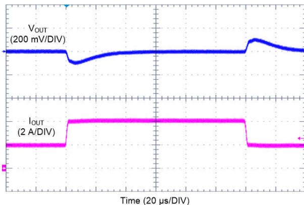
Time (20 µs/DIV) V_{OUT} = 5\text{ V} F_{SW} = 2100\text{ kHz} AUTO Mode I_{OUT} = 2\text{ A to } 4\text{ A to } 2\text{ A} V_{IN} = 13.5\text{ V} T_R = T_F = 2\mu\text{s}
