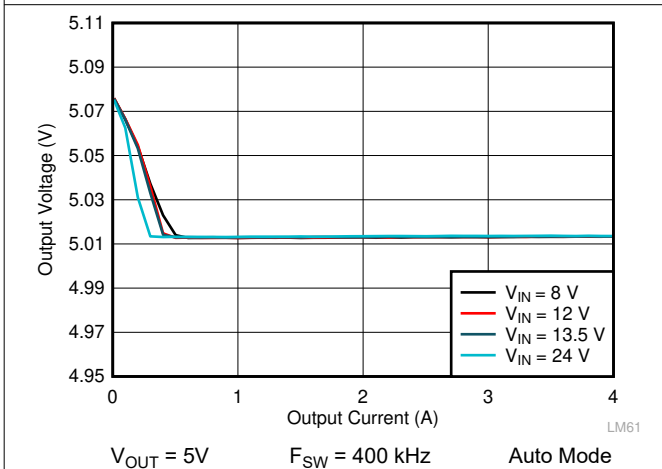
图 10-13. LM61440-Q1 Load and Line Regulation
