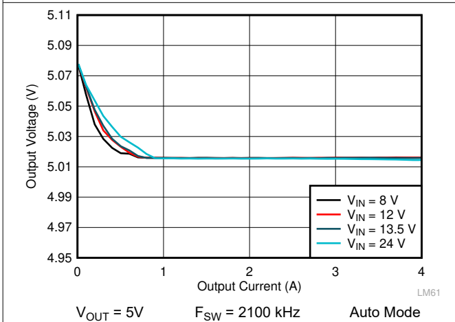
图 10-15. LM61440-Q1 Load and Line Regulation
