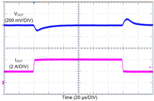
Time (20 µs/DIV) V_{OUT} = 3.3\text{ V} F_{SW} = 400\text{ kHz} AUTO Mode I_{OUT} = 2\text{ A to } 4\text{ A to } 2\text{ A} V_{IN} = 13.5\text{ V} T_R = T_F = 2\mu\text{s}
