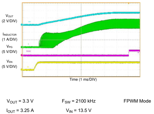
图 9-26. LM61440 Start-up with 3.25-A
