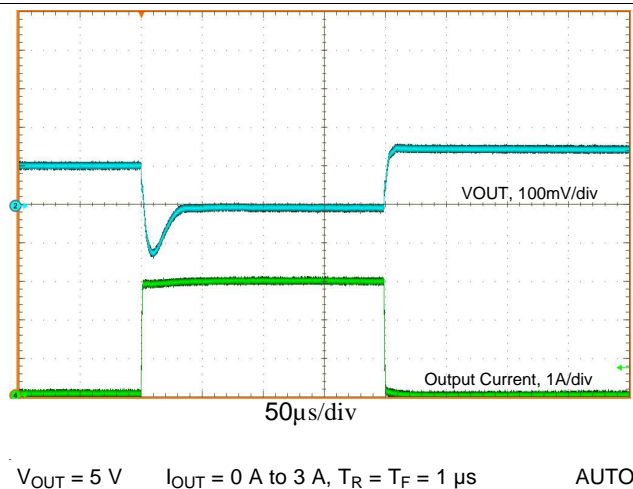
Figure 28. Load Transients
