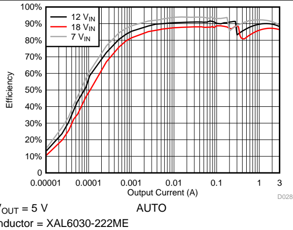
Figure 19. Efficiency
