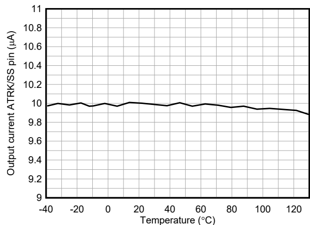
图 6-8. Soft-Start current versus Temperature
