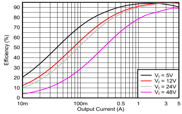
图 10-3. Efficiency Versus I_O (MODE = VCC2 V_O = 12V)
