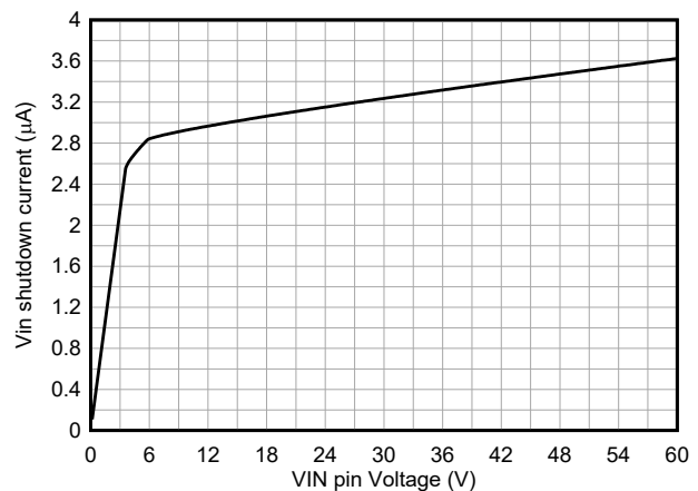
图 6-6. Shutdown Current into VIN versus Pin Voltage V_{EN/UVLO} = 0\text{V} , V_{(VIN)} = 12\text{V} , V_{(BIAS)} = 0\text{V}
