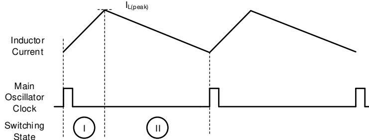
图 8-4. Inductor Current in Continuous Current Boost Operation
