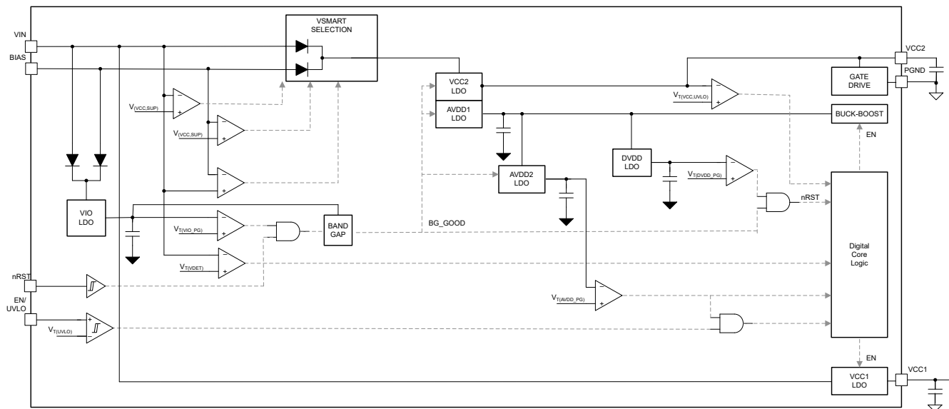
图 8-8. Functional Block Diagram Reference System
