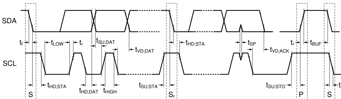
图 8-31. I 2 C Data Transmission Timing
