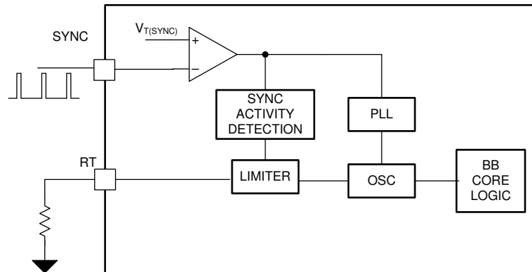
图 8-19. Main Oscillator Functional Block Diagram
