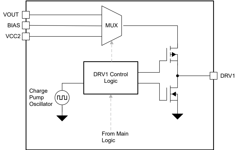
图 8-22. Functional Block Diagram - DRV pin
