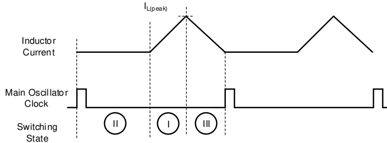
图 8-5. Inductor Current in Continuous Buck-Boost Operation
