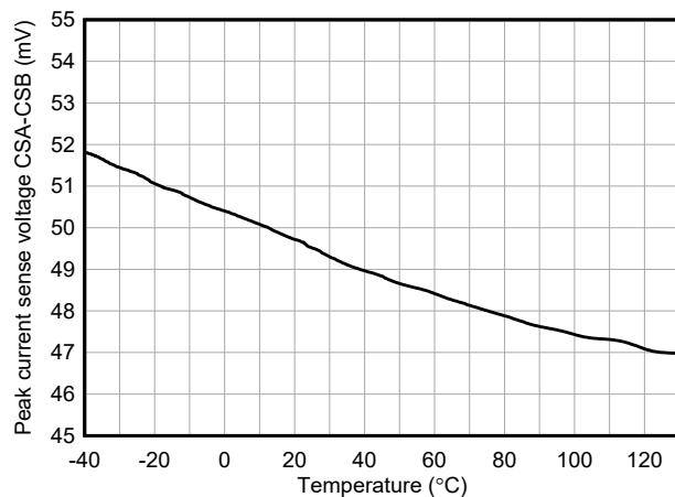
图 6-5. Current Limit Threshold Voltage Versus Temperature
