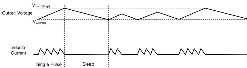
图 8-6. Timing Diagram for the Power Save Mode
