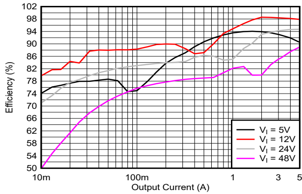
图 10-2. Efficiency Versus I_O (MODE = 0V V_O = 12V)
