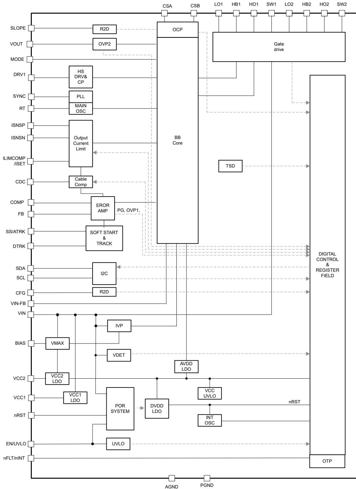
图 8-1. LM51772 Functional Block Diagram
