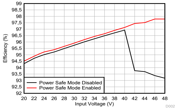
图 10-6. Efficiency Versus V_I ( V_O = 48V, I_O = 5A)
