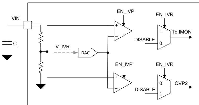
图 8-28. Functional Block Diagram IVP/IVR
