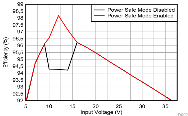
图 10-4. Efficiency Versus V_I ( V_O = 12V, I_O = 5A)
