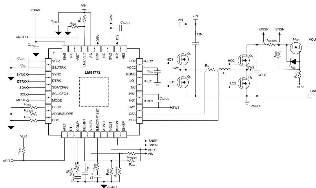
图 10-1. Simplified Schematic of a Typical Application
