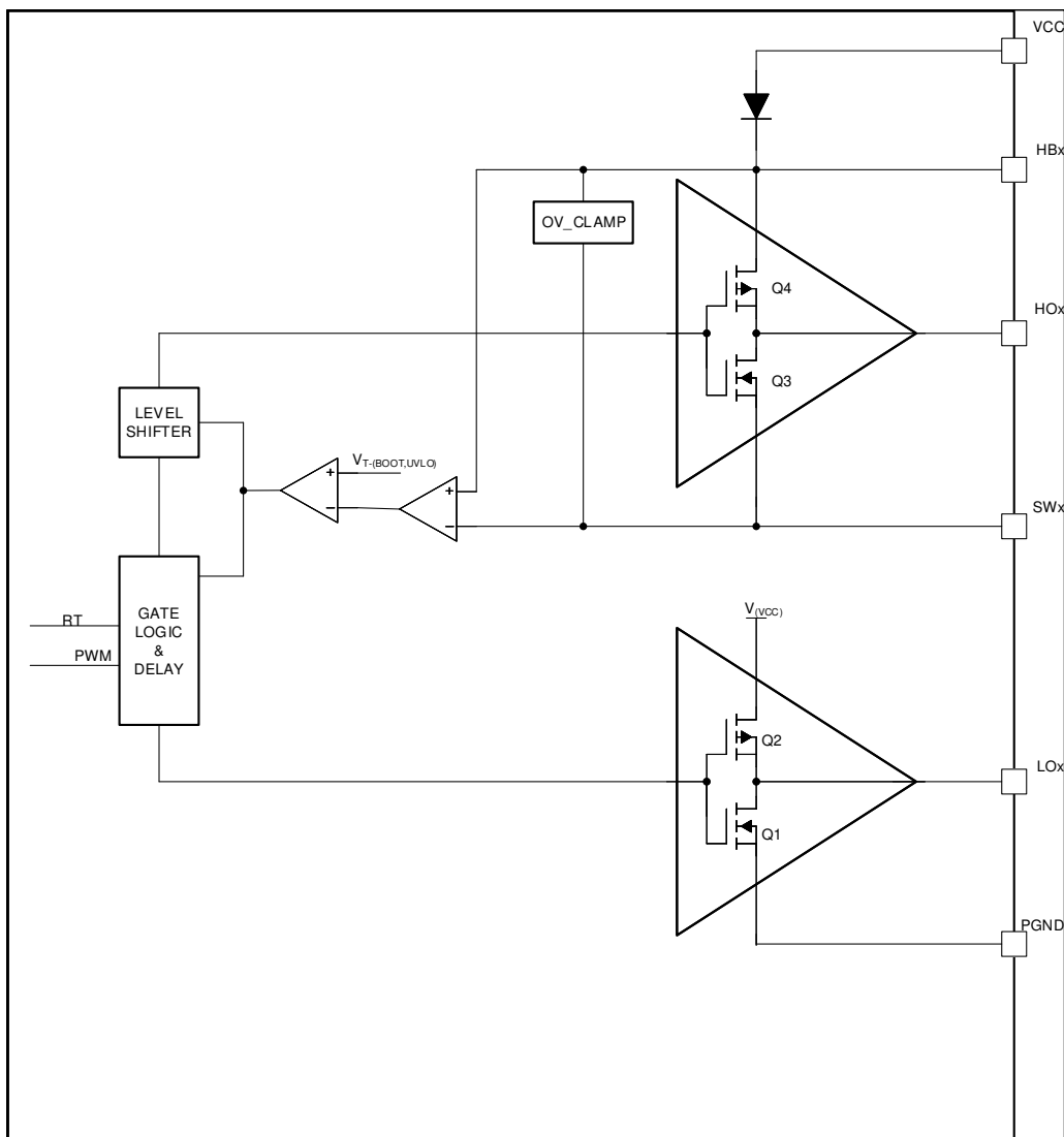
图 8-24. Functional Block Diagram Gate Driver
