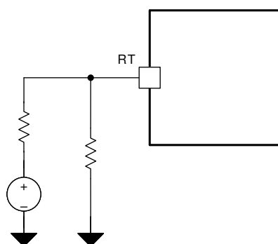
图 8-18. Dynamic Frequency Changing Example
