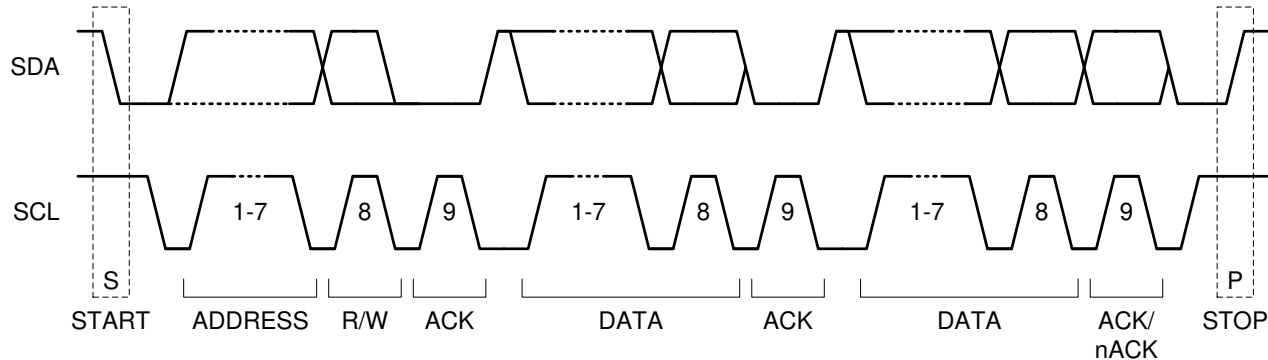
图 8-30. I 2 C START / STOP / ACKNOWLEDGE Protocol
