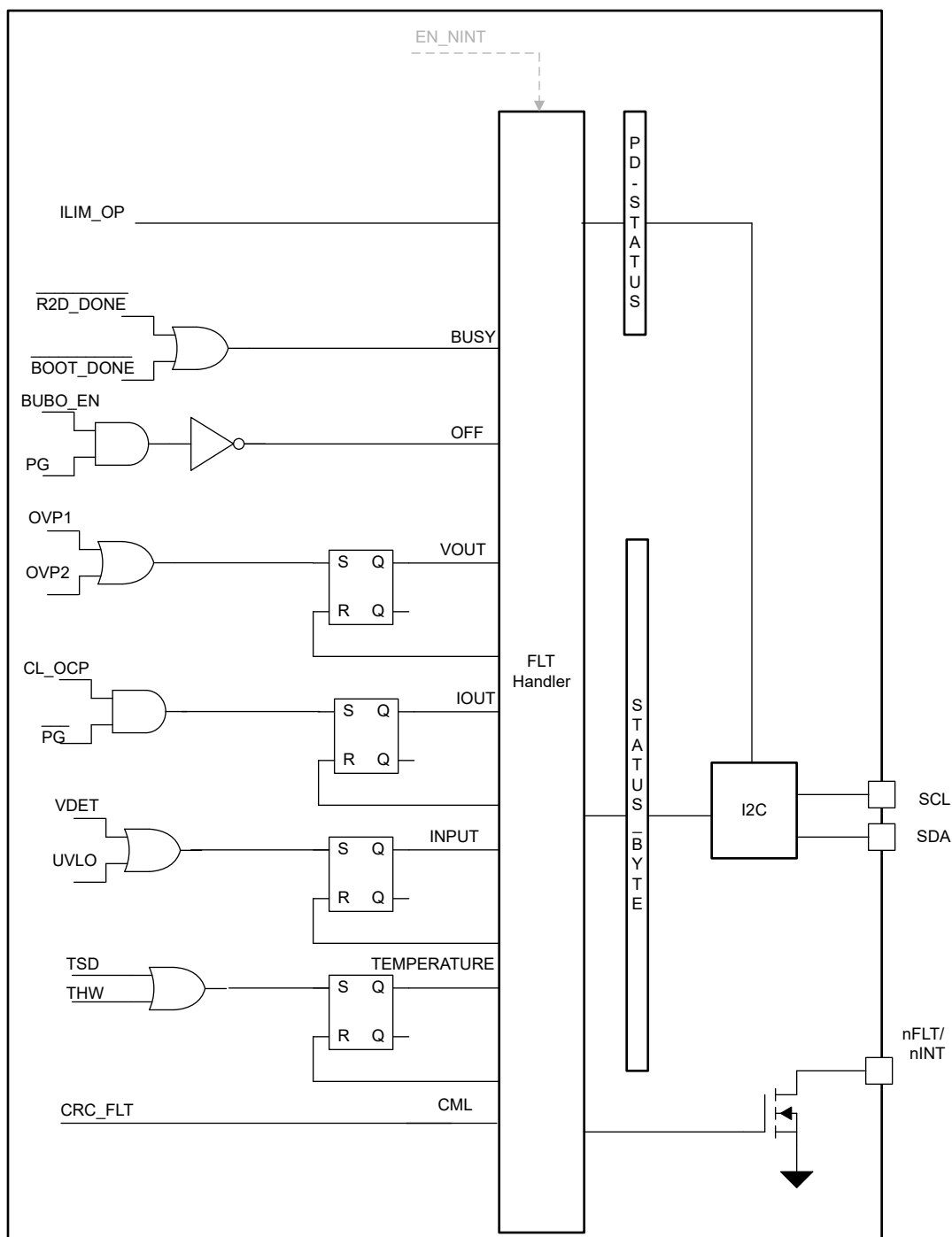
图 8-26. Functional Block Diagram Fault Handler
