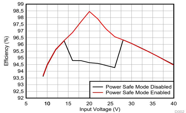
图 10-5. Efficiency Versus V_I ( V_O = 20V, I_O = 5A)
