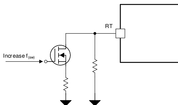
图 8-17. Frequency Hopping Example
