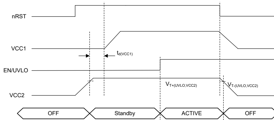
图 8-14. Timing Diagram VCC Regulator
