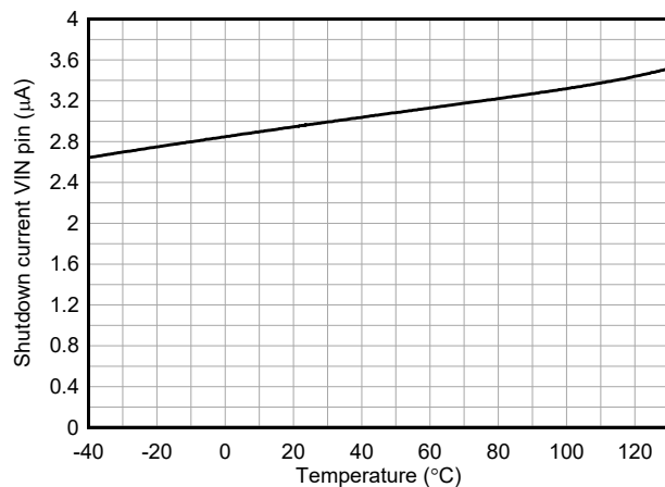
图 6-7. Shutdown Current into VIN versus Temperature V_{EN/UVLO} = 0\text{V} , V_{(VIN)} = 12\text{V} , V_{(BIAS)} = 0\text{V}
