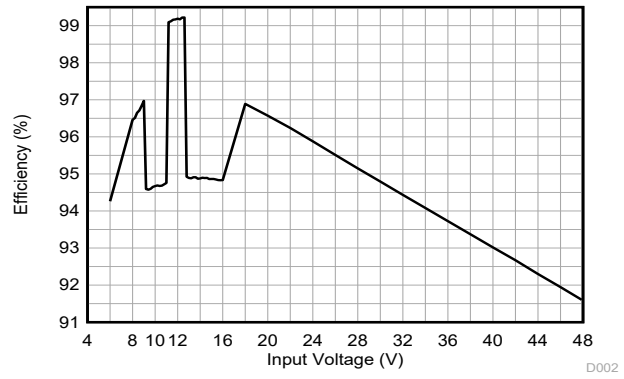
图 10-7. Efficiency Versus V_I ( V_{PCM,low} = 11V, V_{PCM,high} = 13V, I_O = 5A, MODE = VCC2)
