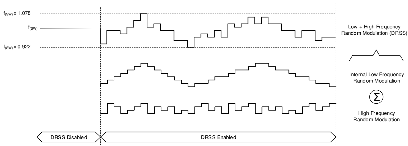
图 8-23. Dual Random Spread Spectrum
