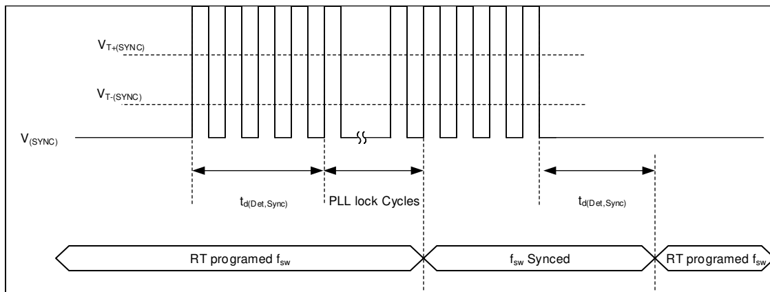
图 8-20. Timing Diagram SYNC Function
