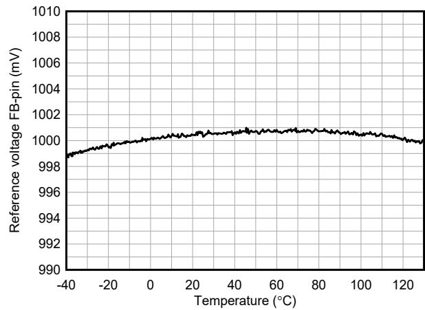
图 6-4. FB Pin Reference Voltage versus Temperature
