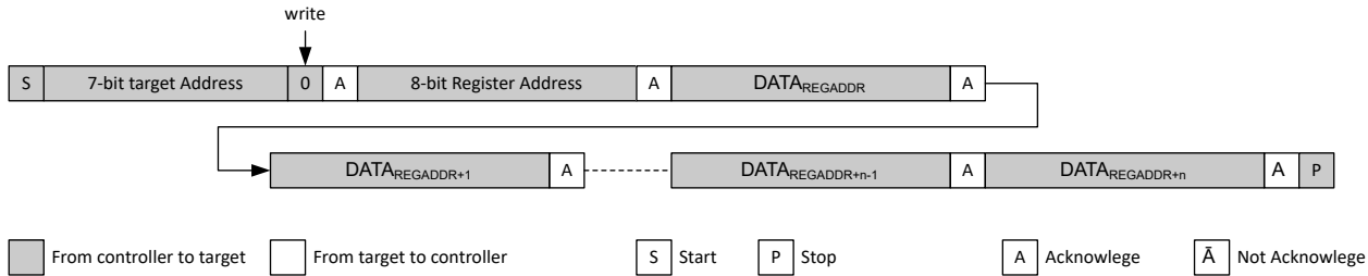
图 8-36. Sequential WRITE starting at a defined register address
