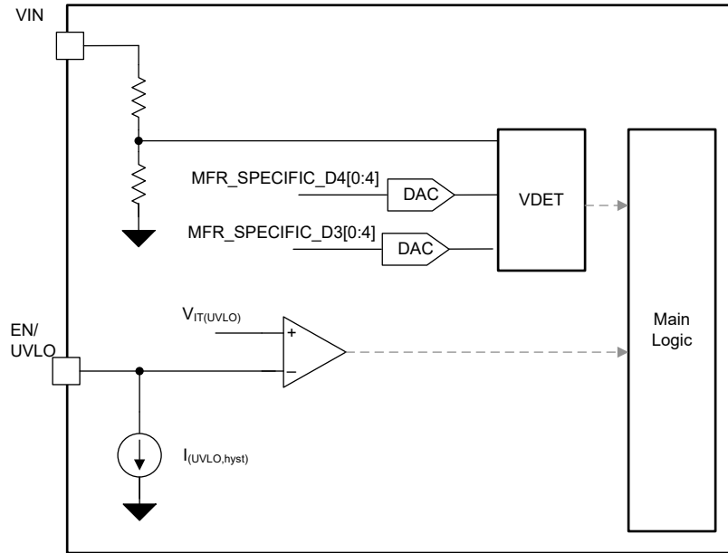
图 8-12. Functional Block Diagram UVLO and VDET
