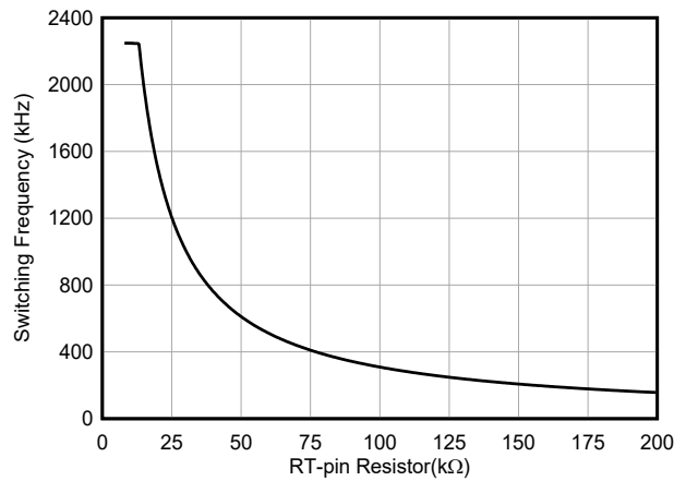
图 6-3. Switching Frequency Versus RT Resistance
