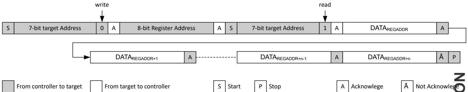
图 8-34. Sequential READ starting from a defined register address
