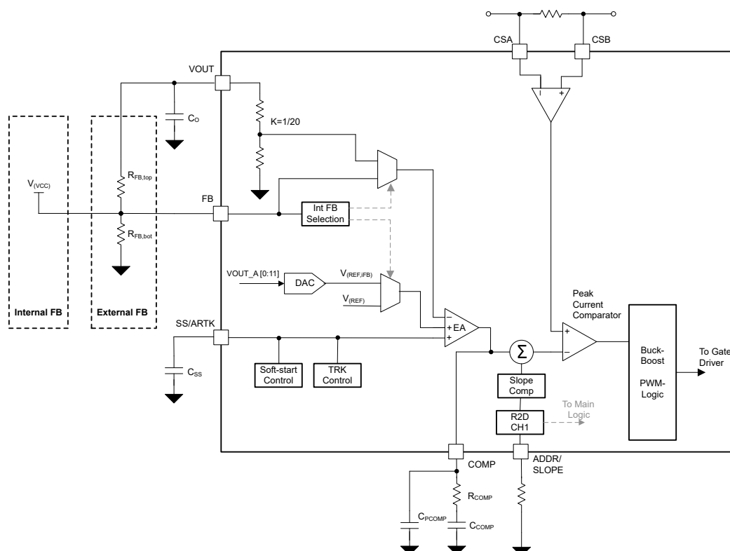
图 8-15. EA Functions Block Diagram
