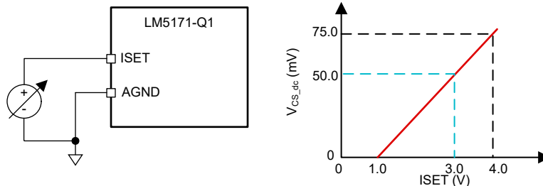
图 7-3. Analog Voltage Channel Current Programming
