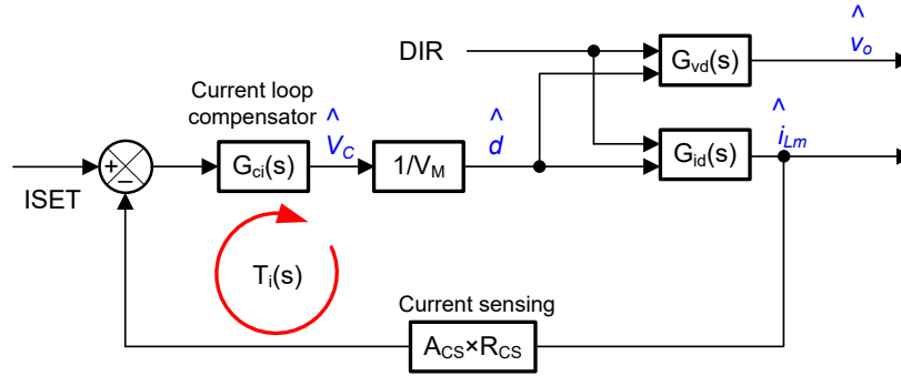
图 8-2. Current Loop Block Diagram
