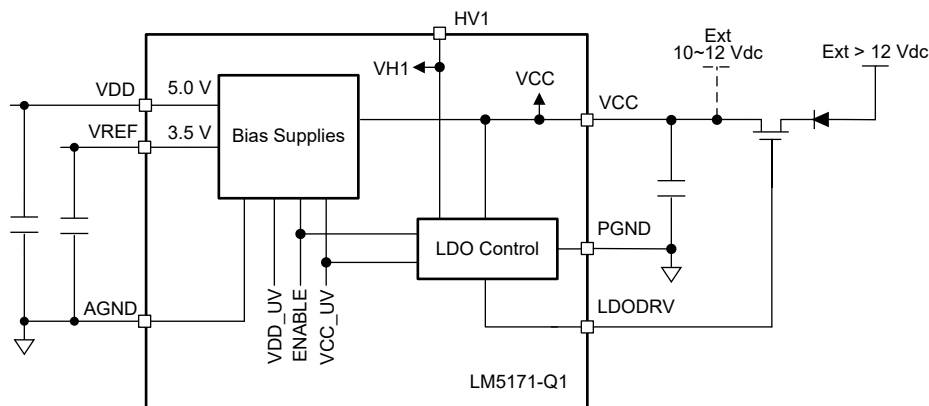
图 7-1. Bias Supplies Connections
