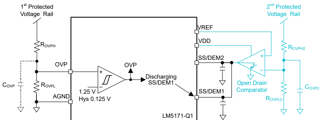
图 7-23. OVP for 2nd Protected Voltage Rail in Multiphase Parallel Operation
