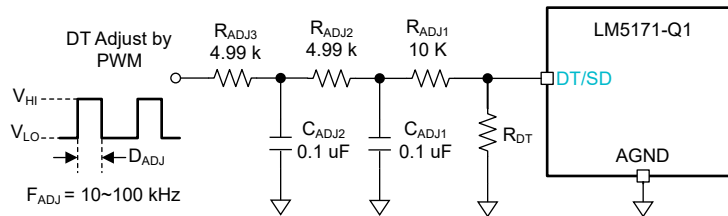
图 7-30. Dynamic Dead Time Adjustment b
