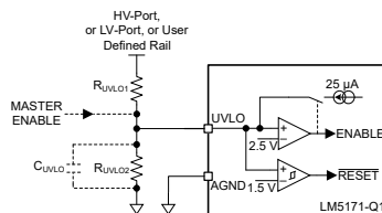
图 7-31. UVLO Programming
