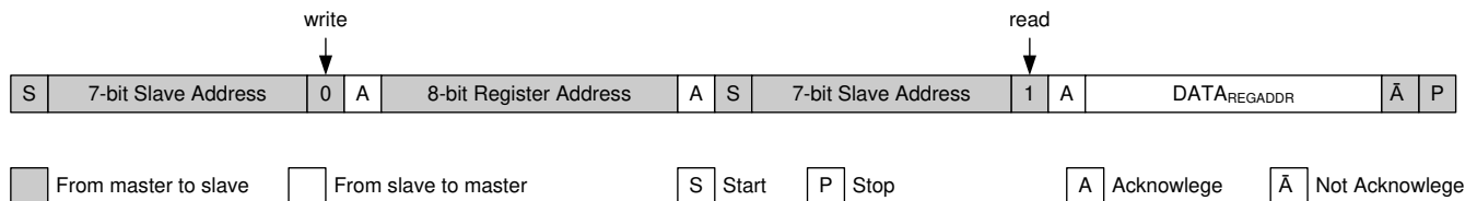
图 7-36. Single READ From a Defined Register Address
