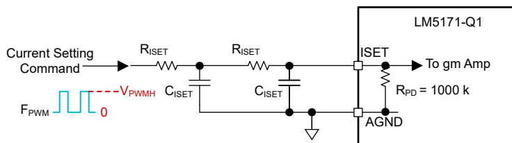
图 7-4. PWM Channel Current Programming
