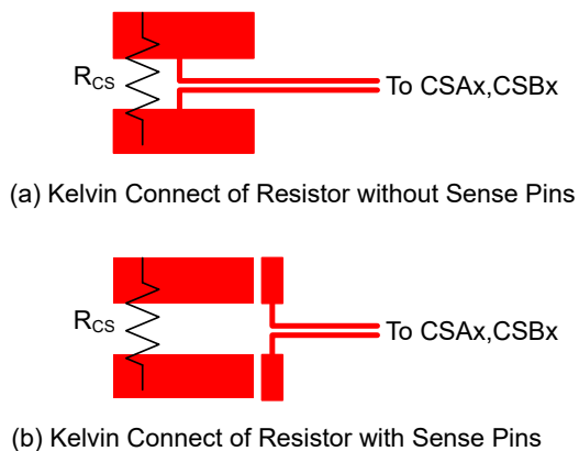
图 8-26. A Layout Example of Current Sense Routing
