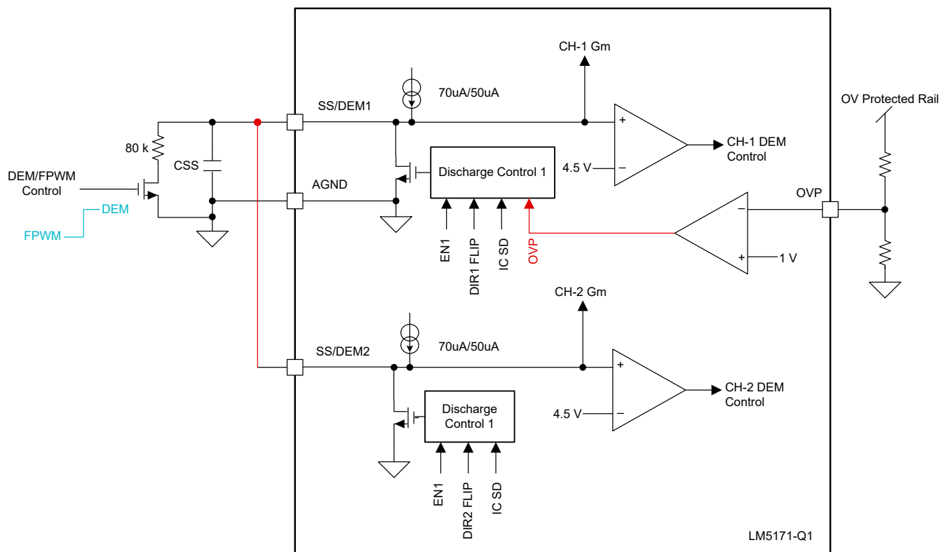
图 7-12. OVP Implementation for SS-DEM Pins Connection for Parallel Operation
