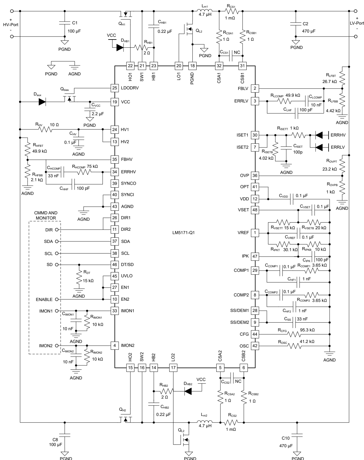
图 8-6. Schematic of the Example Dual-Phase Bidirectional Converter
