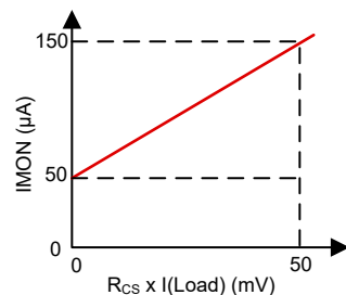
图 7-6. IMON Current Source vs Boost Load Current
