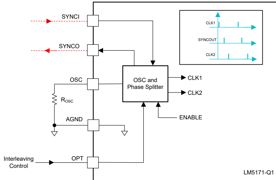
图 7-21. Oscillator and Interleaving Clock Programming
