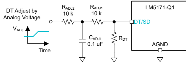
图 7-29. Dynamic Dead Time Adjustment A
