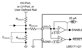
图 7-32. UVLO With Additional Hysteresis Programming
