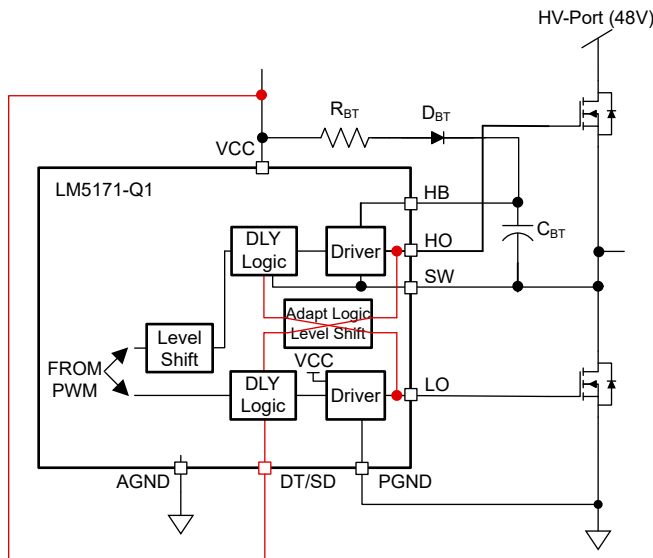
图 7-17. Dead Time Programming With DT Pin (Only One Channel is Shown)
