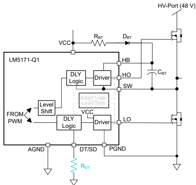
图 7-15. Dead Time Programming With DT Pin (Only One Channel is Shown)
