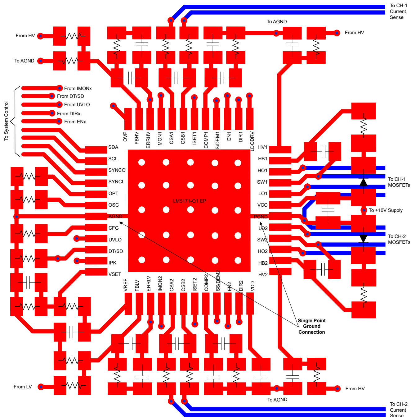
图 8-27. A Layout Example of LM5171-Q1 Critical Signal Routing
