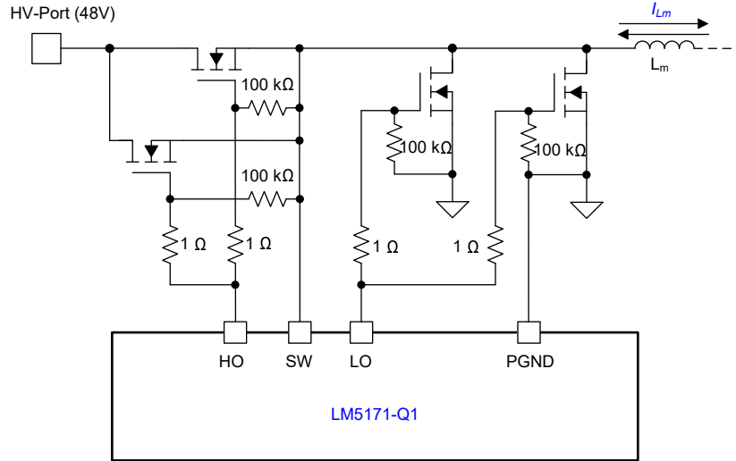
图 8-8. Paralleled MOSFET Configuration
