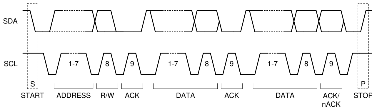
图 7-33. I 2 C START / STOP / ACKNOWLEDGE Protocol
