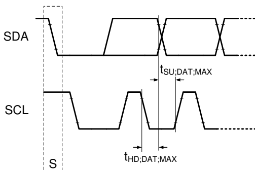
图 7-35. I 2 C Data Transmission Timing for maximum rise/fall times.
