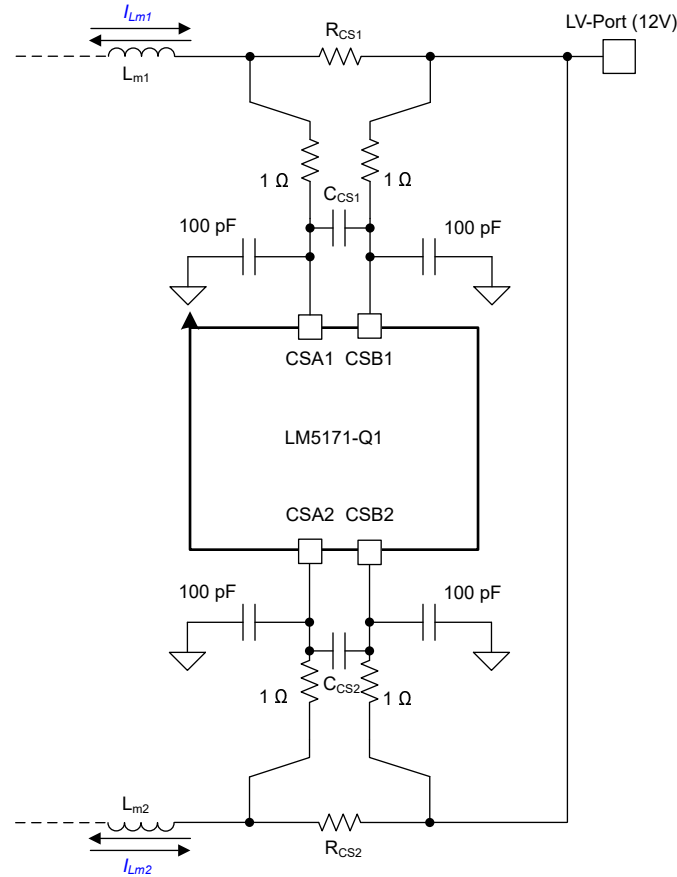
图 8-7. Current Sense With RC filter
