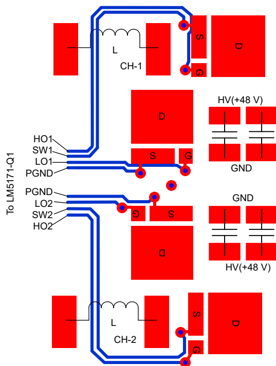
图 8-25. A Layout Example of MOSFET Gate Drive Routing
