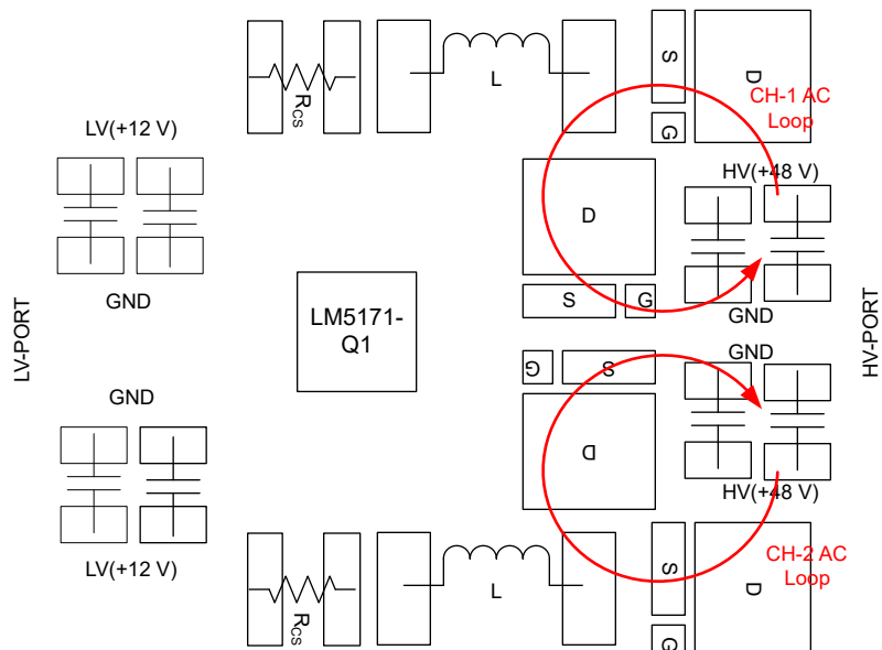
图 8-24. A Layout Example of Dual-Channel Power Circuit Placement
