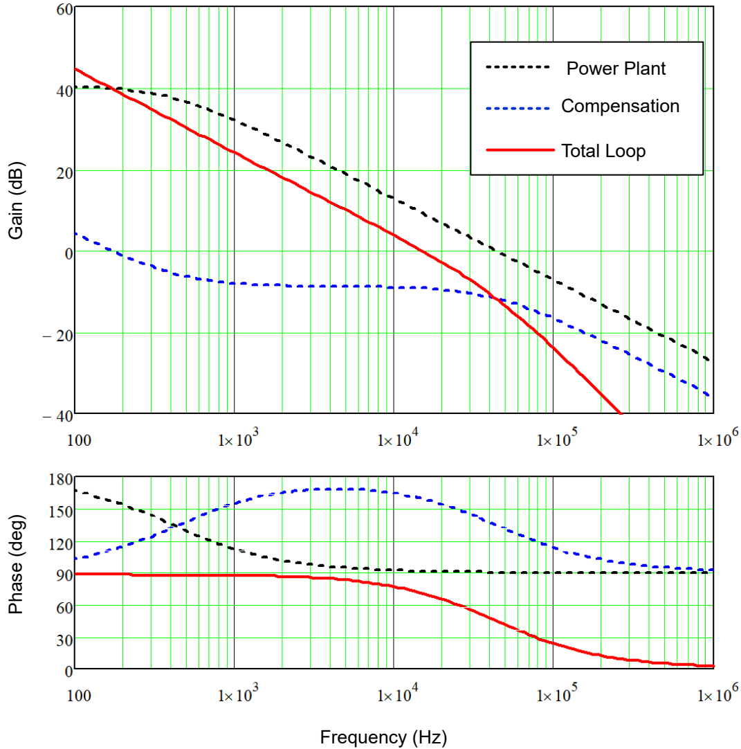
图 8-10. Bode Plots of the current loop
