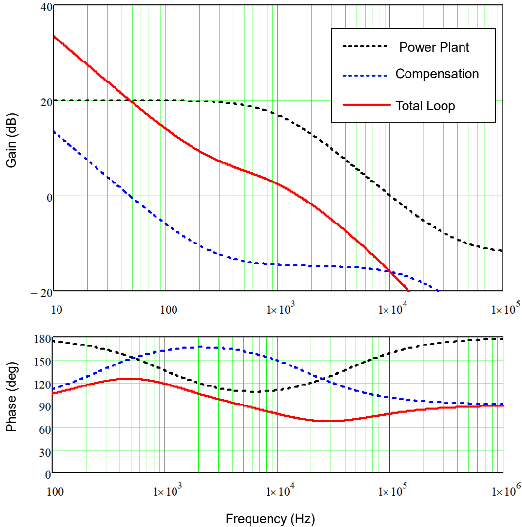
图 8-11. Bode Plots of the current loop
