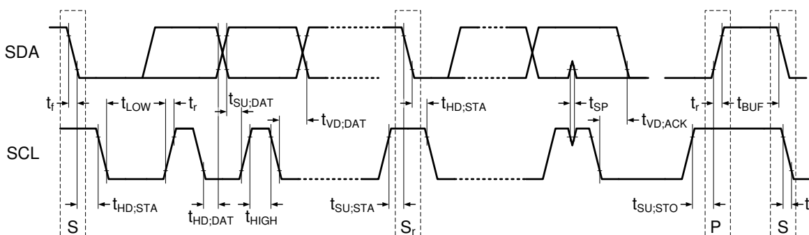
图 7-34. I 2 C Data Transmission Timing
