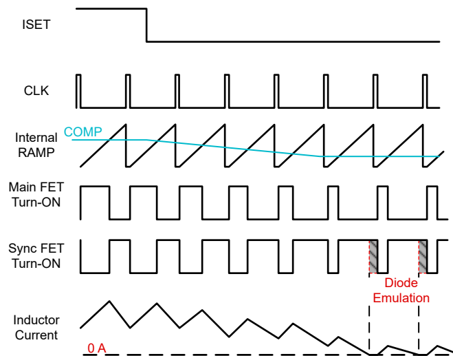
图 7-11. Diode Emulation Operation
