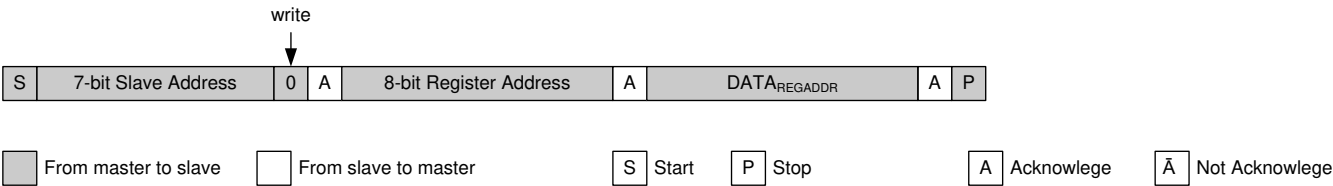
图 7-38. Single WRITE to Defined Register Address
