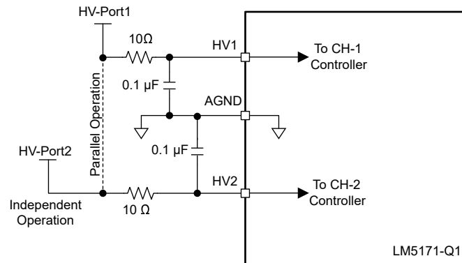
图 7-2. HV1 and HV2 Pins Configuration
