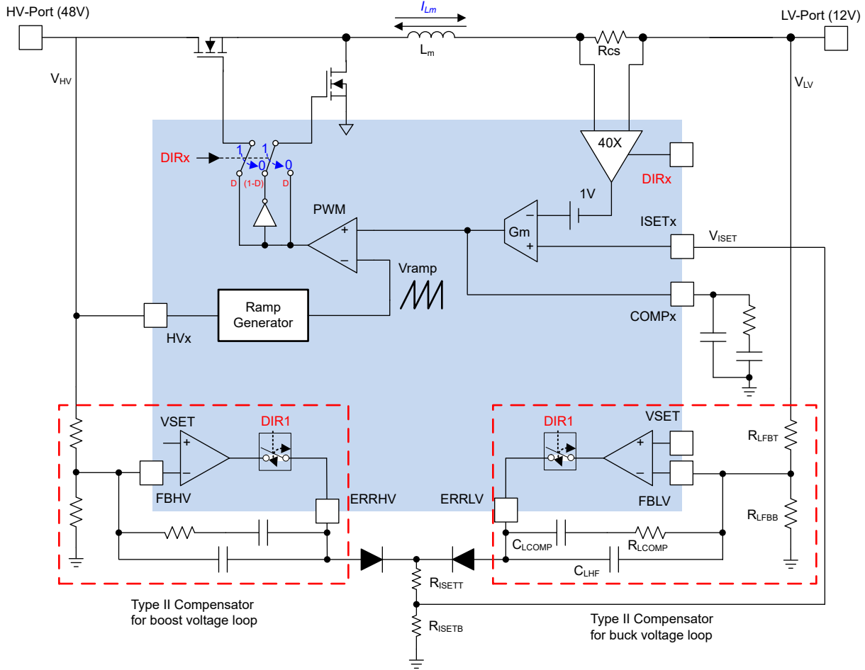
图 8-5. Outer Voltage Loop Control
