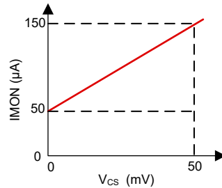
图 7-5. IMON Current Source vs Current Sense Voltage
