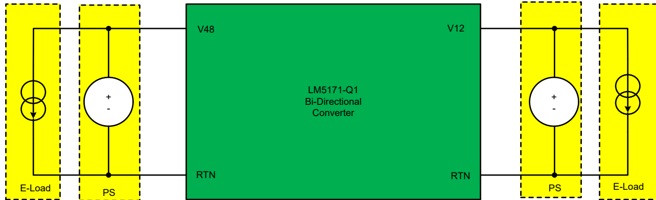
图 8-23. Emulated Dual Battery System With Bench Power Supplies and E-Loads
