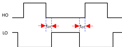
图 7-16. Gate Drive Dead Time (Only One Channel is Shown)
