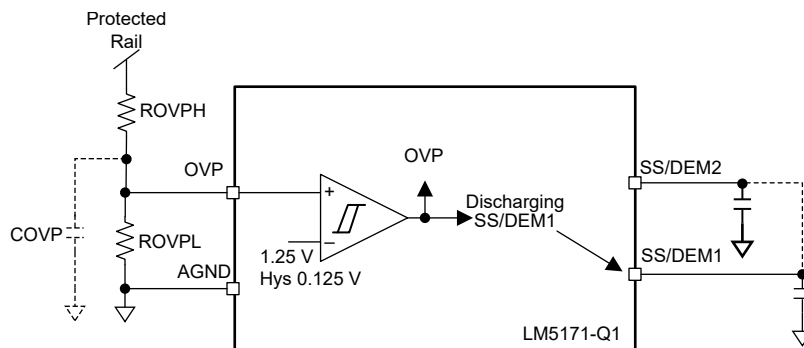
图 7-22. OVP for CH-1 or Multiphase Parallel Operation
