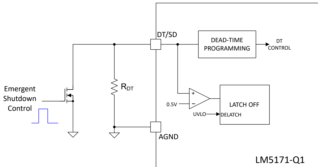
图 7-19. Emergent Latched Shutdown
