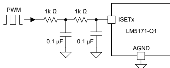
图 8-12. Two-Stage RC Filter to Convert the PWM into an Analog Voltage at the ISETx Pin
