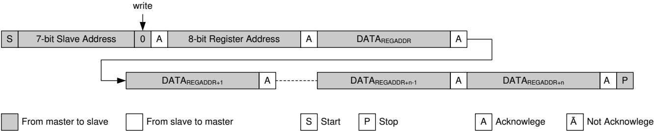
图 7-39. Sequential WRITE Starting At A Defined Register Address
