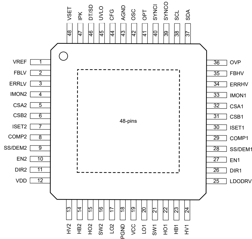
图 5-1. PHP Package 48-Pin TQFP Top View
