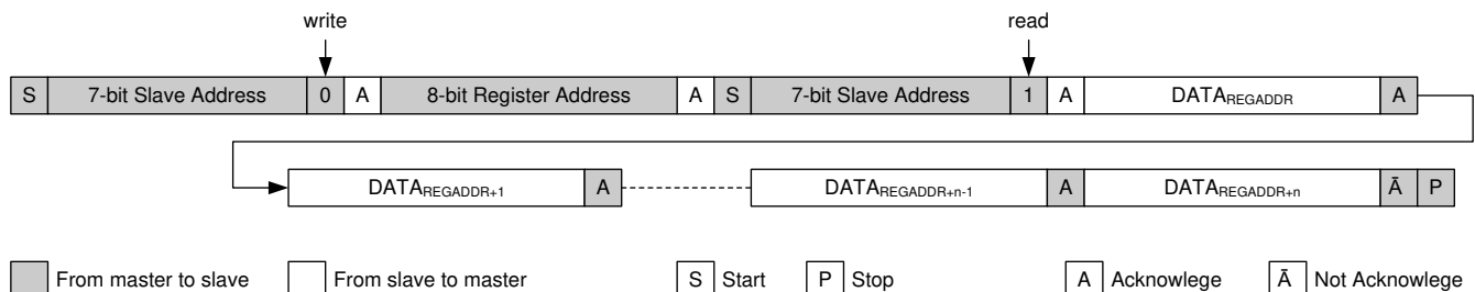
图 7-37. Sequential READ Starting From A Defined Register Address
