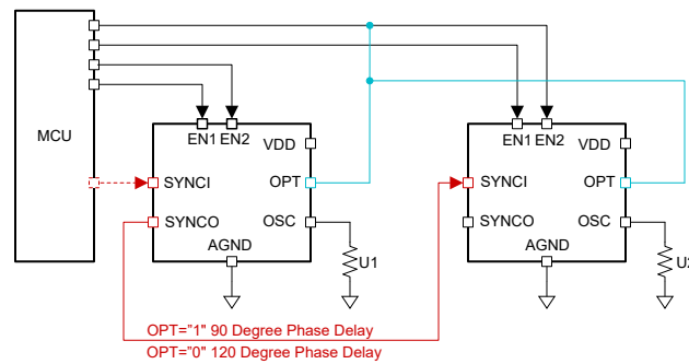
图 7-25. Three or Four Phases Interchangeable Configuration
