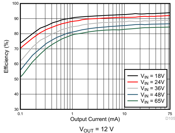
图 8-22. Efficiency
