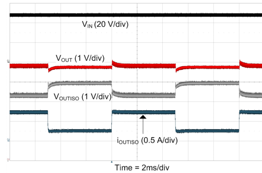
图 38. Secondary Load Transient at I_{ISO} = 250 mA - 750 mA
