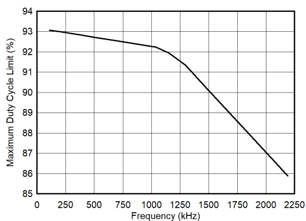
图 7-16. Maximum Duty Cycle Limit vs Frequency
