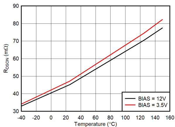
图 7-14. Internal MOSFET Drain Source On-state Resistance vs Temperature
