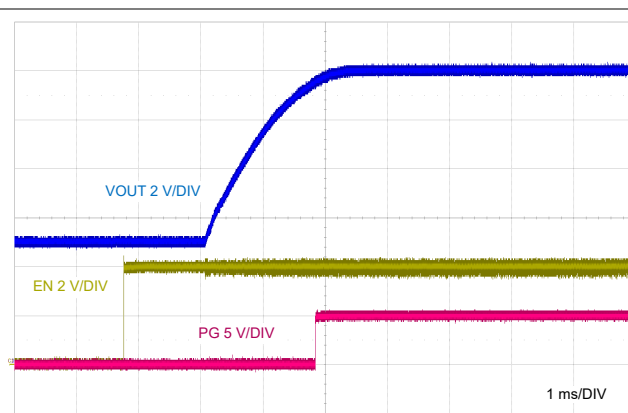
图 9-26. EN Start-Up Pre-bias Characteristic
