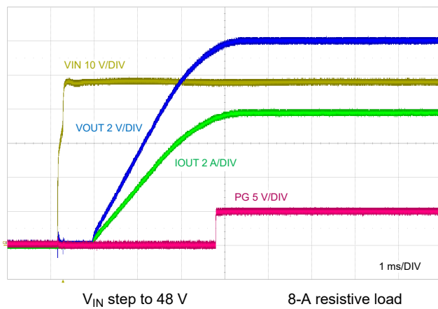
图 9-23. Start-Up Characteristic
