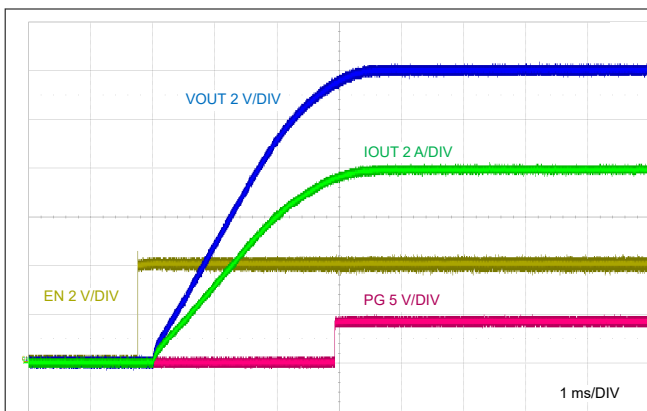
图 9-24. EN Start-Up Characteristic
