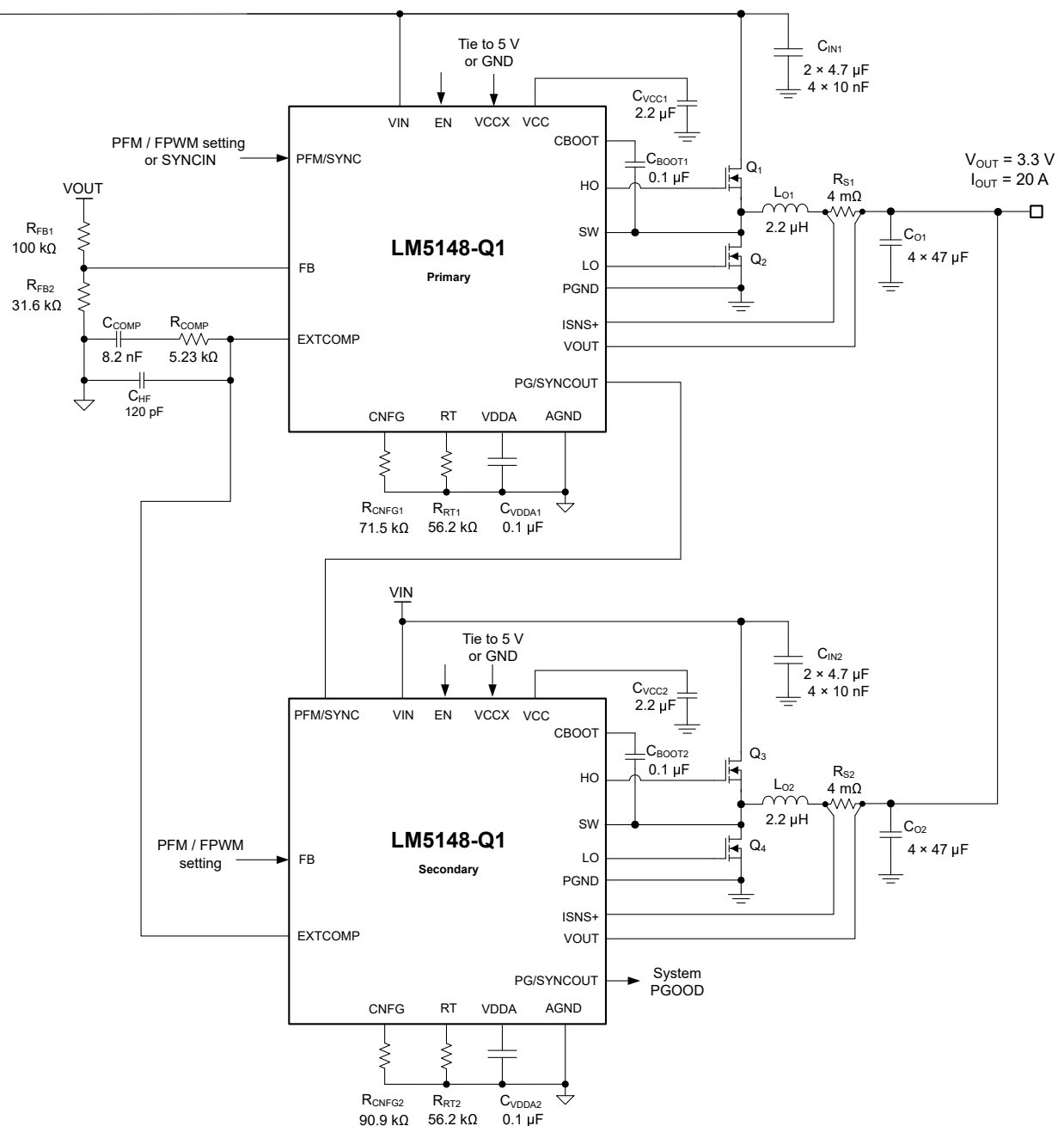
图 9-39. Application Circuit 4 with Two LM5148-Q1 Buck Regulators Switching at 400 kHz
