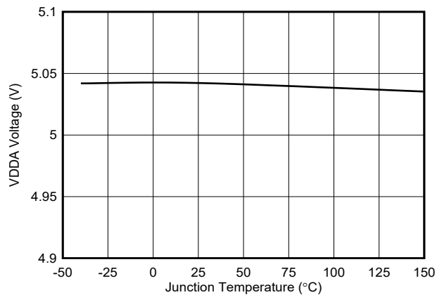
图 7-14. VDDA Regulation Voltage vs Temperature
