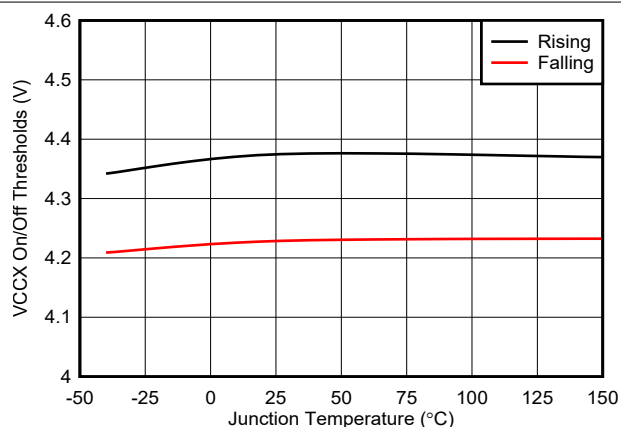
图 7-16. VCCX On, Off Thresholds vs Temperature
