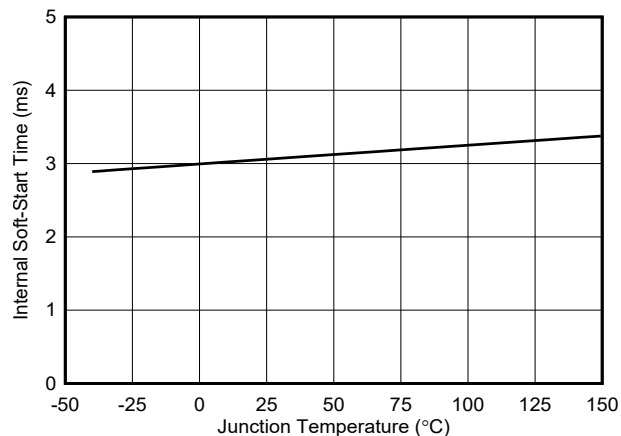
图 7-20. Soft-Start Time vs Temperature
