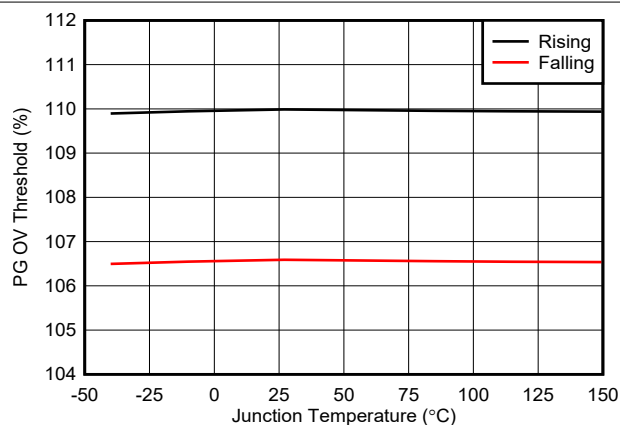
图 7-9. PG OV Thresholds vs Temperature
