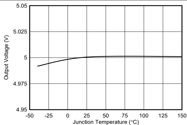
图 7-7. Fixed 5-V Output Voltage vs Temperature
