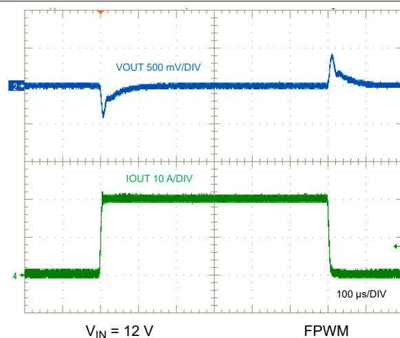
图 9-45. Load Transient, 0 A to 20 A
