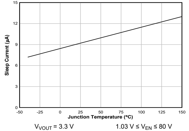
图 7-4. Sleep1 Current vs Temperature
