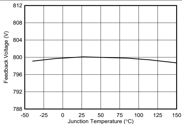
图 7-8. Feedback Voltage vs Temperature
