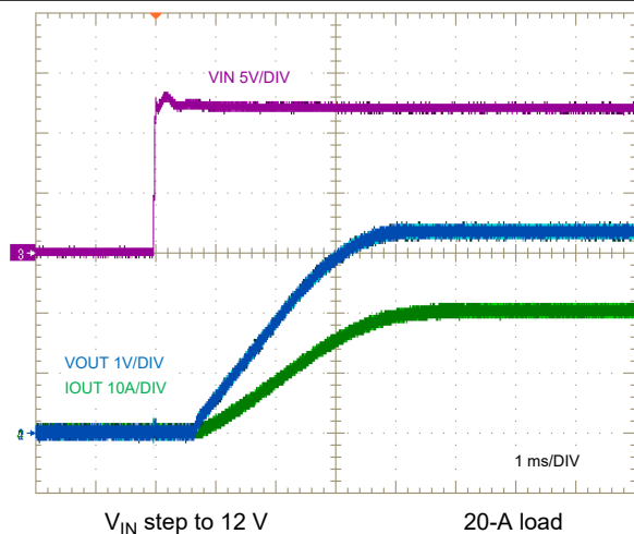
图 9-42. V_{IN} Start-Up Characteristic
