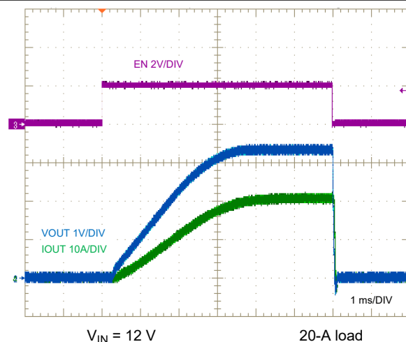
图 9-43. ENABLE ON and OFF Characteristic
