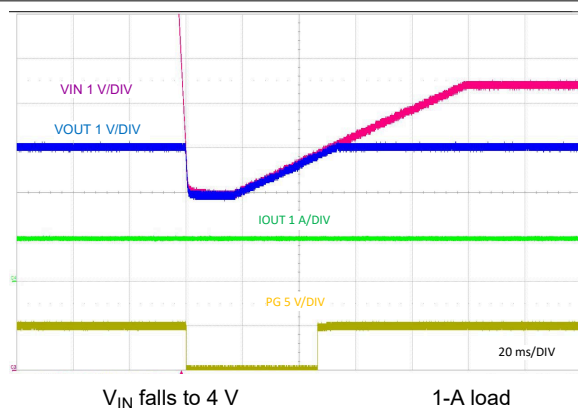
图 9-34. Cold-Crank Response to V_{IN} = 4 V
