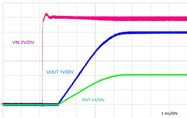
图 9-35. Start-Up Characteristic
