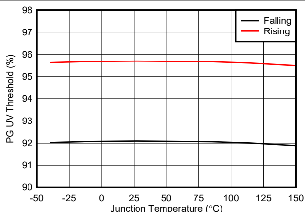
图 7-10. PG UV Thresholds vs Temperature
