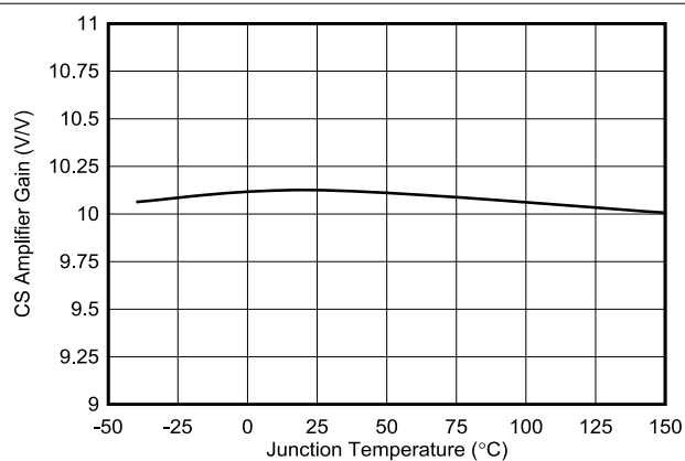
图 7-18. Current Sense (CS) Amplifier Gain vs Temperature
