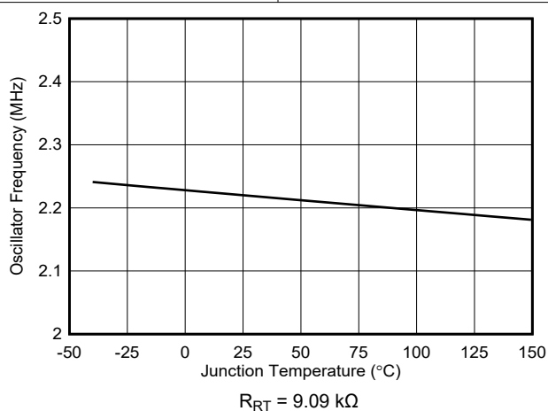
图 7-21. Switching Frequency vs Temperature
