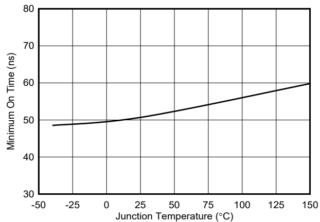
图 7-19. Minimum On Time (HO) vs Temperature
