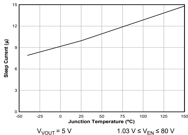
图 7-5. Sleep2 Current vs Temperature
