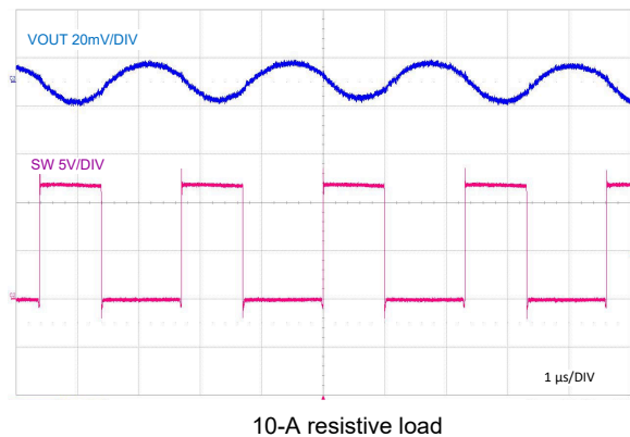
图 9-31. Full Load Switching
