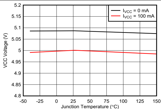
图 7-11. VCC Regulation Voltage vs Temperature
