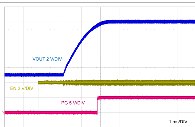
图 9-25. EN Start-Up Pre-bias Characteristic
