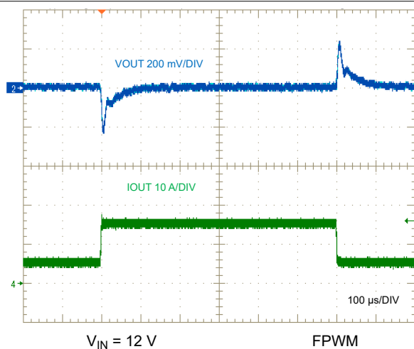
图 9-44. Load Transient, 5 A to 15 A
