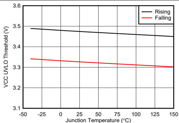
图 7-12. VCC UVLO Thresholds vs Temperature
