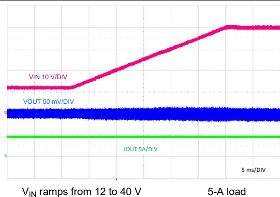
图 9-33. Line Transient Response to V_{IN} = 40 V
