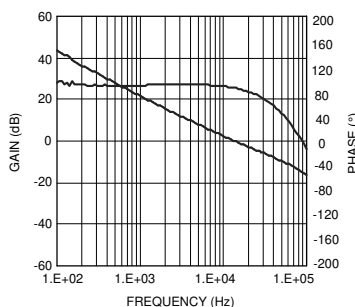
图 8-6. Overall Loop Gain and Phase
