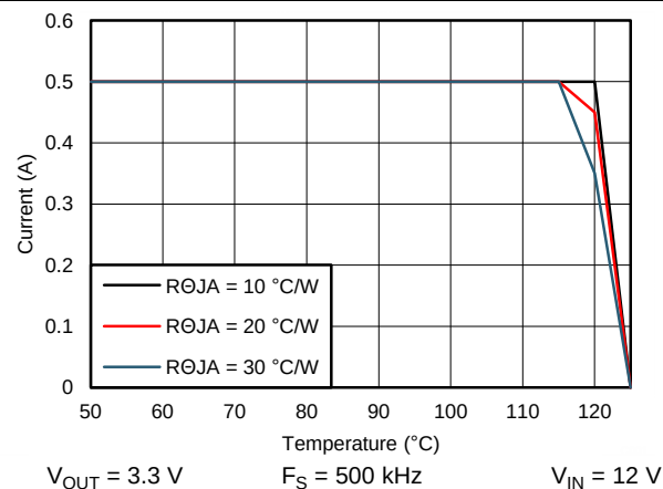
Figure 58. Derating Curve
