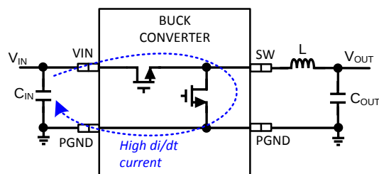
Figure 106. Buck Converter High di / dt Path
