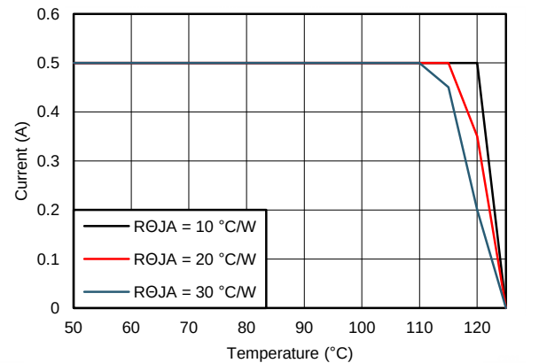
Figure 76. Derating Curve
