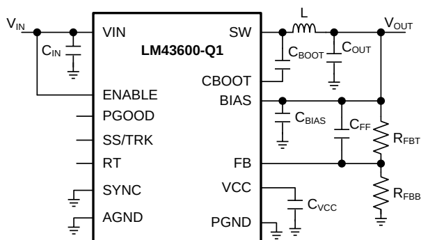
Figure 44. LM43600-Q1 Basic Schematic for V_{OUT} \geq 3.3 V, Tie BIAS to V_{OUT}
