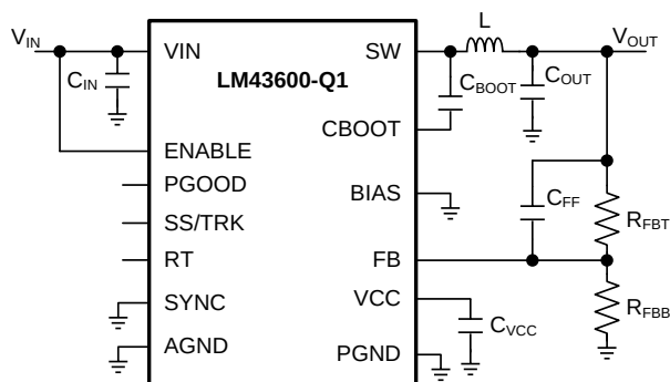
Figure 45. LM43600-Q1 Basic Schematic for V_{OUT} < 3.3 V, Tie BIAS to Ground
