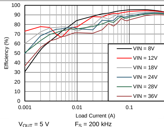
Figure 66. Efficiency
