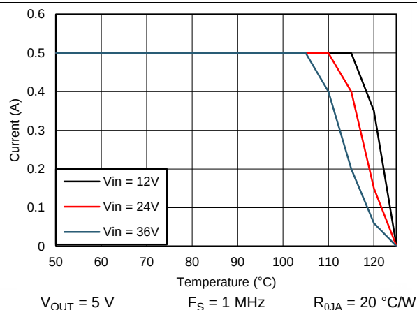
Figure 92. Derating Curve with R_{\theta JA} = 20^\circ\text{C/W}
