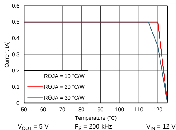
Figure 70. Derating Curve
