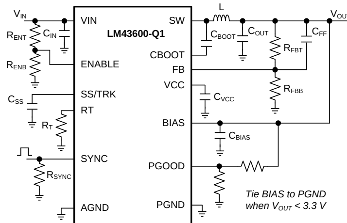
Figure 46. LM43600-Q1 Schematic with All Features
