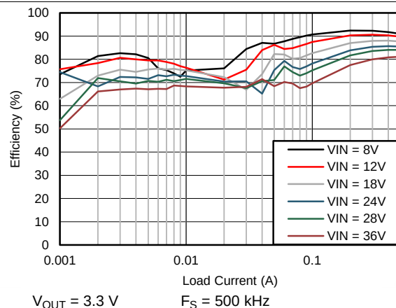
Figure 54. Efficiency
