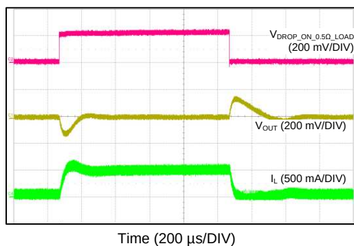
Figure 63. Load Transient Between 0.05\text{ A} and 0.5\text{ A}
